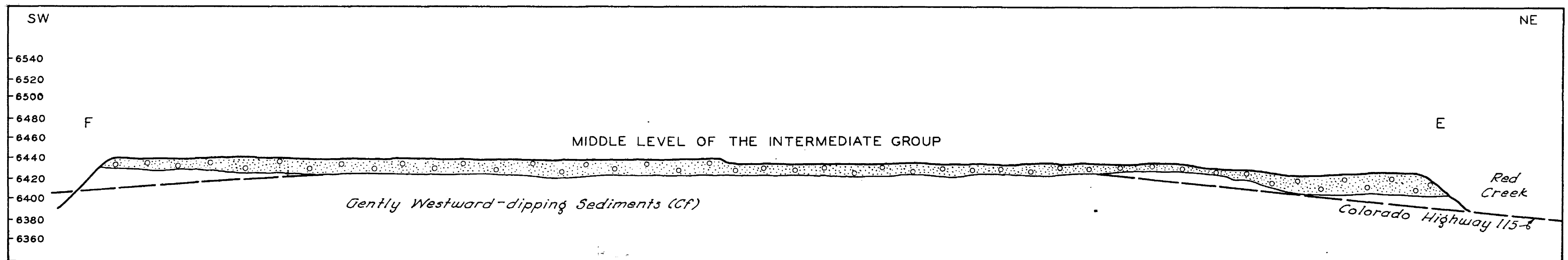
FIGURE 2. SHOWING CROSS-SECTIONS THROUGH ROCK CREEK SURFACES OF THE LOW LEVEL GROUP AND RED CREEK SURFACE OF THE INTERMEDIATE GROUP ALONG COLORADO HIGHWAY 115. THE LOCATION OF THESE SECTIONS IS INDICATED BY THE APPROPRIATE LETTERS ON PLATE 1. NOTE THE CHANNEL-LIKE IRREGULARITIES IN THE OTHERWISE SMOOTH BEDROCK SURFACE.
