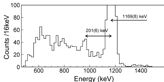
Fig. 1. The energies of decay signals within 1–16 ms after the implantation of ^{141}\text{Ho} ions. An energy difference of 201(6) keV was obtained for two observed proton peaks, the known transition at 1169(8) keV [13] and the peak at 0.97 MeV corresponding to a proton transition to the 202.1 keV 2^+ level in ^{140}\text{Dy} [16].
