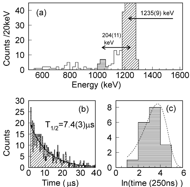
Fig. 2. (a) Energy spectrum of ^{141m}\text{Ho} decay signals between 0.5 and 40 \mu\text{s} after the recoil implantation. The energy difference of 204(11) keV between two observed peaks was determined using the calibration procedure based on the known 959.7(28) keV proton line from ^{113}\text{Cs} [26,27] and verified using known 1235(9) keV ^{141m}\text{Ho} proton peak [15]. Shaded areas correspond to the energy gates used in the lifetime analysis. The 1.17 MeV proton emission from 4.1 ms ^{141g}\text{Ho} resulted in about 20 counts present in the spectrum at the left side of the 1235 keV line. Panel (b) shows the decay pattern of the main peak together with the exponential fit yielding a more precise value of T_{1/2} = 7.4(3) \mu\text{s} microseconds for ^{141m}\text{Ho} . (c) Decay pattern of the 1.03 MeV line (horizontally hashed) together with predicted shape for the T_{1/2} = 7.4 \mu\text{s} decay.
