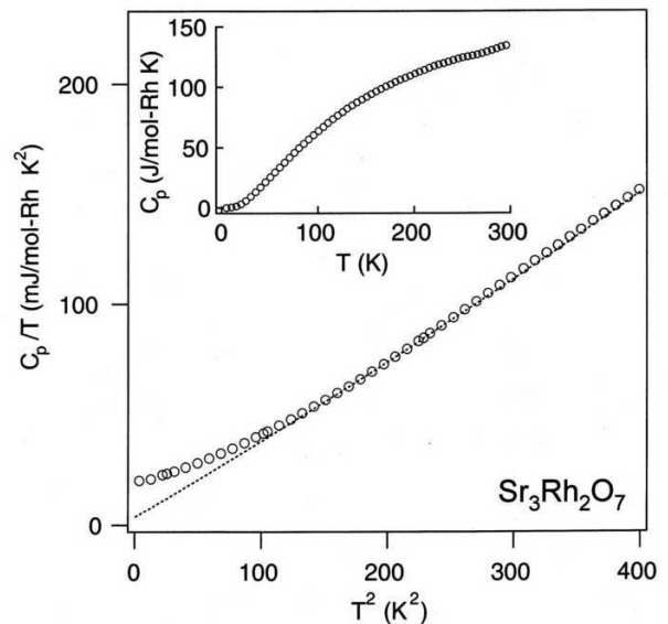
FIG. 6: Specific heat of the polycrystalline \text{Sr}_3\text{Rh}_2\text{O}_7 . The data are plotted in C_p/T vs T^2 (main panel) and C_p vs T (inset) forms. The dotted curve represents a fit to the data (details are in the text).
