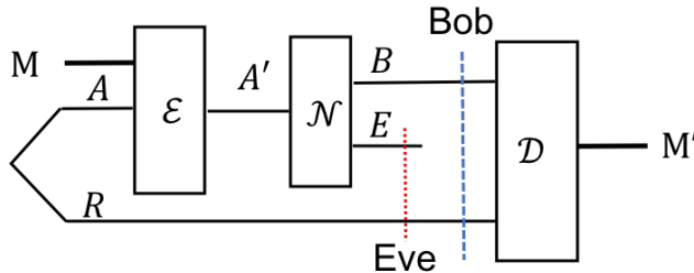
Figure 2: The information-processing task for EA private communication through a quantum channel \mathcal{N} . Bob, who has access to the systems R and B , can reliably decode the transmitted message. However, Eve, who has access systems R and E , can only get negligible information about Alice’s message.
