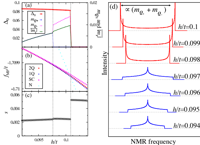
FIG. 3: Mean-field solutions for t'/t = 0.2 , V/t = 0.8 , J/t = 2.4 , and T/t = 0.003 with L = 432 . (a) Order parameters ( \Delta_0 , m_{Q+} , and m_{Q-} ) and the spatially-averaged magnetization \overline{|m_r|} . (b) Free energy densities f_{MF}/t for different solutions of self-consistent equations (2). (c) Entropy s (computed by taking the derivative of the free energy density as a function of temperature) as a function of magnetic field. (d) Expected shape of the NMR spectrum, see text for details.
