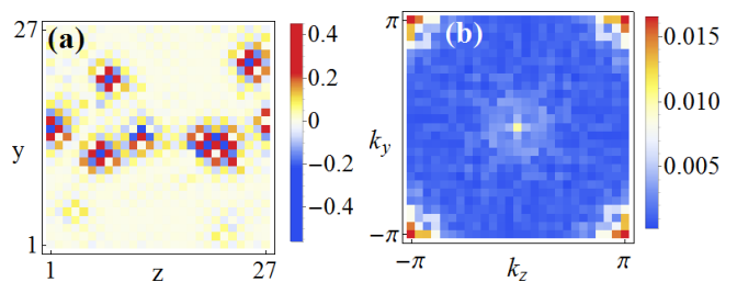
FIG. 7. (a) Magnetization in real space for the set of unrelaxed Z-impurities used in Fig. 5. (b) The Fourier transform of (a) clearly showing the absent sharp \mathbf{Q} peaks of the corresponding relaxed system in Fig. 5(c).
