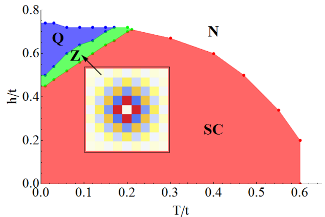
FIG. 4. Phase diagram of the inhomogeneous system displaying an extended Q-phase where isolated magnetic Z-impurities (oriented along the z axis, with J_z S_{i^*}^z = 20 ) locally nucleate magnetization with the same local structure as in the magnetically long-range ordered Q-phase, i.e. along the x axis.
