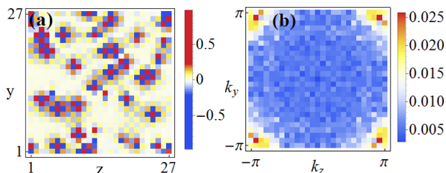
FIG. 6. (a) Real space m^x(r) component induced by a relaxed system of 5% X-impurities ( j_x S_i^x = 20 ) in the absence of an external magnetic field ( H = 0 ). (b) Averaged |m^x(\mathbf{q})| including three different configurations, exhibiting sharp peaks at \mathbf{Q}_{\pm} arising from cooperative exchange.
