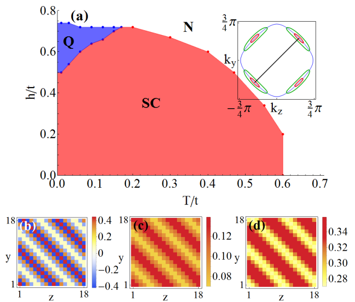
FIG. 1. (a) Phase diagram of the clean system including the Q-phase (blue region) at low T and high magnetic fields H , the d -wave SC phase (red region), and the non-SC non-magnetic normal N phase (white region). The inset shows the normal state electron-like Fermi surface (blue curve) and two sets of contours of constant quasiparticle energy at h = \{0.22, 0.5\} (red, green) along with the nesting vector \mathbf{Q}_+ (black line). (b-d) Self-consistent magnetic m^x(r) , m^z(r) , and superconducting \Delta(r) order parameters in the Q-phase, at h = 0.7 and T = 0.01 .
