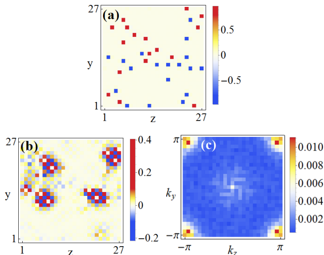
FIG. 5. (a) Real space m^z(r) component for a relaxed sample system of 5% Z-impurities ( j_z S_i^z = 20 ) in the absence of an external magnetic field ( H = 0 ). The corresponding FT is simply noise. (b) Induced magnetization m^x(r) for the same system. (c) Averaged |m^x(\mathbf{q})| including three of these Z-impurity configurations.
