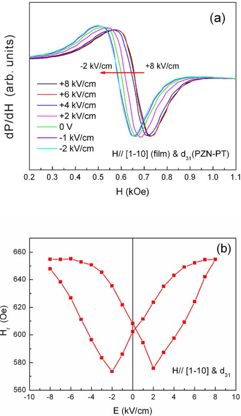
Fig. 8 (a) Variation of FMR absorption derivative with magnetic field for different electric field strengths, and (b) FMR field as a function of electric field strength applied across the PZN-PT crystal, while an applied magnetic field is aligned along the [1-10] of the film and the d_{31} direction of PZN-PT crystal.
