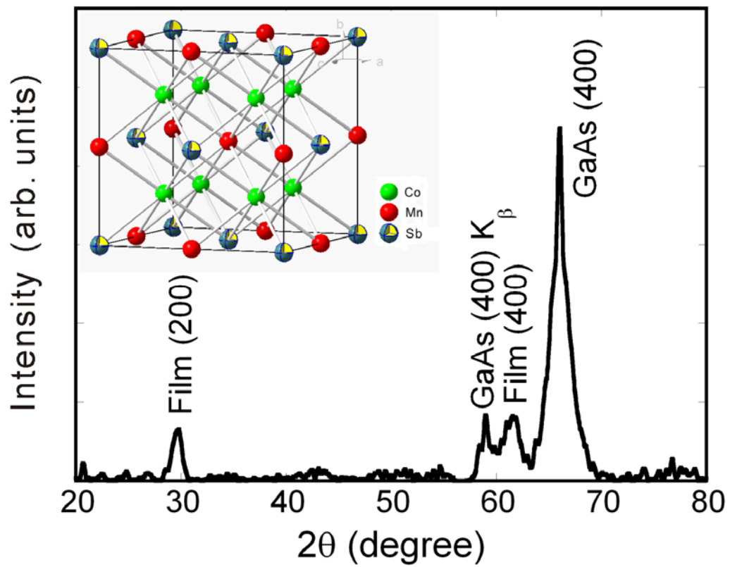
Fig.3 XRD spectrum of Co 2 MnSb film. Inset illustrates a L 21 type structure.
