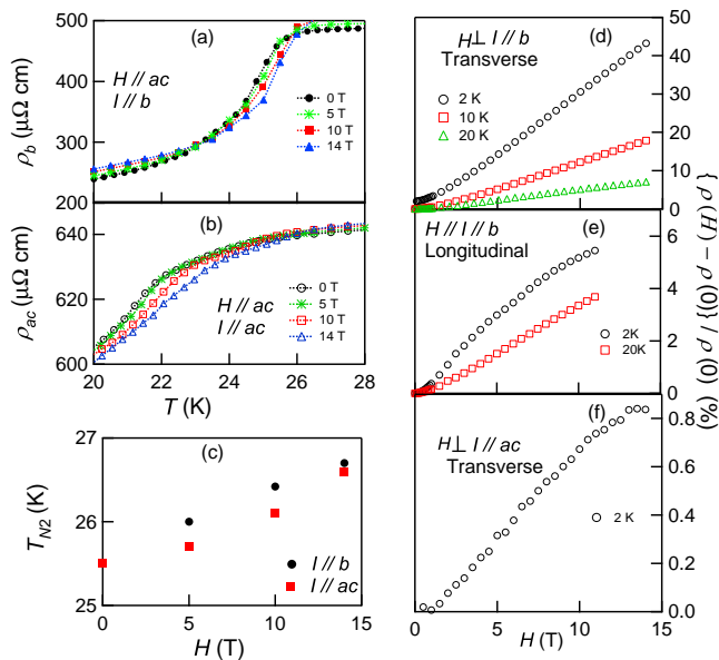
FIG. 3: Temperature dependence of \rho_b (a) and (b) \rho_{ac} of \text{CaFe}_4\text{As}_3 between 20 and 28 K at indicated applied magnetic fields. The dotted lines are guides to eyes. (c) Variation of T_{N2} with the applied magnetic field, which is obtained at points where \rho_b and \rho_{ac} drop 10 percent compared to that extended from high-temperature resistivity. (d) Transverse magnetoresistivity along the b axis ( H \perp I \parallel b ), (e) longitudinal magnetoresistivity along the b axis ( H \parallel I \parallel b ) (e), and (f) transverse magnetoresistivity in the ac plane ( H \perp I \parallel ac ).
