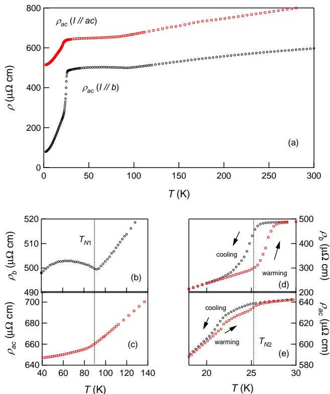
FIG. 2: (a) Temperature dependence of electrical resistivity \rho_b and \rho_{ac} of \text{CaFe}_4\text{As}_3 along the b axis and the ac plane, respectively. \rho_b and \rho_{ac} near T_{N1} \sim 90 K are highlighted in (b) and (c), respectively. (d) and (e) show thermal hysteresis in \rho_b and \rho_{ac} around \rho_{ac} at T_{N2} \sim 26 K, respectively.
