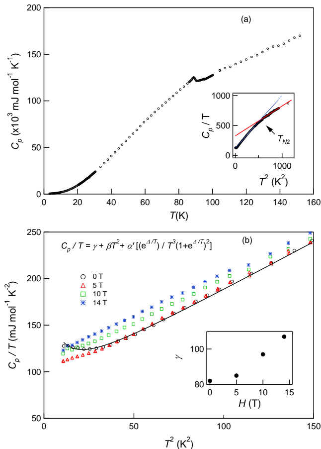
FIG. 7: (a) Temperature dependence of specific heat C_p of \text{CaFe}_4\text{As}_3 . Inset: The change in the slope of C_p/T vs. T^2 at T_{N2} . (b) C_p/T vs. T^2 in the range of 2 to 15 K at indicated magnetic fields. The solid line is the fit of zero-field C_p/T to Eq. (2). Inset: variation of \gamma with H .
