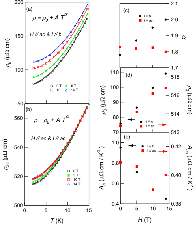
FIG. 5: Temperature dependence of \rho_b (a) and (b) \rho_{ac} of \text{CaFe}_4\text{As}_3 in the range of 2 to 15 K at indicated magnetic fields. The solid lines are fits to the Eq. (1). (c) - (e) show magnetic field dependence of \alpha , \rho_0 , and A , respectively.
