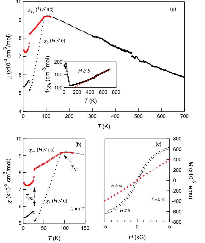
FIG. 6: (a) Temperature dependence of magnetic susceptibilities, \chi_b(T) with H \parallel b , and \chi_{ac}(T) with H \parallel ac for \text{CaFe}_4\text{As}_3 denoted by \bullet and \diamond (color online), respectively. Data between 2 and 400 K were taken at 1 Tesla in a SQUID magnetometer and taken at H = 10 T between 300 to 700 K using a VSM. Inset: Temperature dependence of 1/\chi_b in the range of T = 2 to 700 K. The solid line is a fit to \chi(T) = T / (T - \theta_{CW}) between 400 and 700 K. (b) Magnetic susceptibility \chi_b(T) and \chi_{ac}(T) for T = 2 to 150 K at H = 1 T with AFM SDW transitions at T_{N1} \sim 90 K and T_{N2} \sim 26 K. (c) M vs. H for \text{CaFe}_4\text{As}_3 at 5 K.
