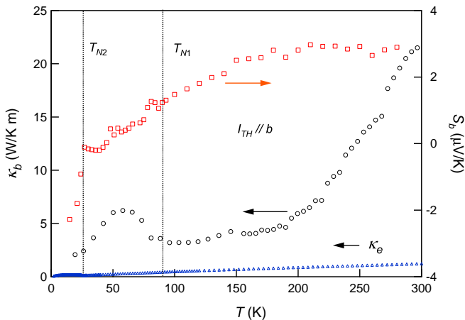
FIG. 8: Thermal conductivity (left axis) and Seebeck coefficient (right axis) of a \text{CaFe}_4\text{As}_3 single crystal for T = 15 to 300 K. For comparison, the estimated electronic thermal conductivity \kappa_e is also plotted.
