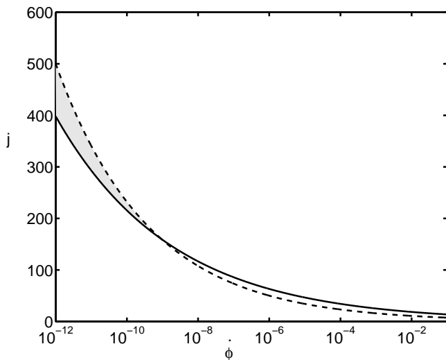
FIG. 4: Analytic results for FRIED quantization with l = 3/4 and initial conditions \phi_i = 0 and \dot{\phi}_i > 0 . The horizon problem is solved in the region above the solid line and the kinetic bound is satisfied below the dashed line. The shaded area represents the region of parameter space that leads to successful inflation for this set of initial conditions.
