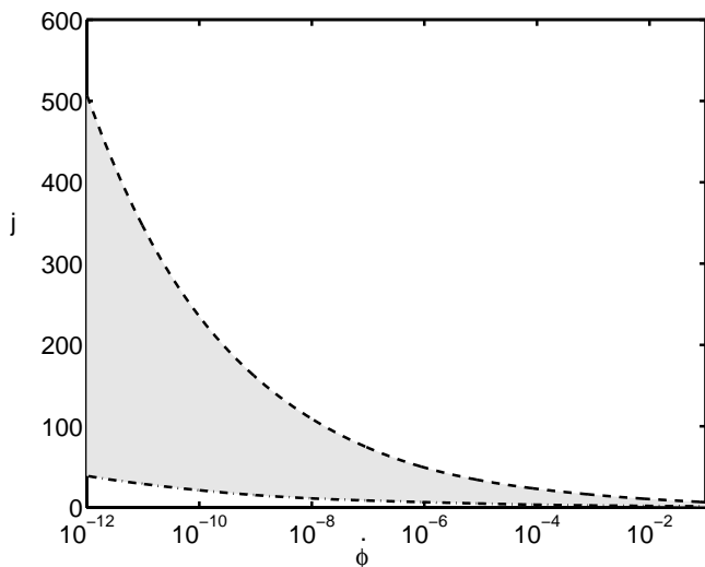
FIG. 7: Numerical results for FRIED quantization with l = 3/4 , where the initial value of the inflaton is determined by imposing the uncertainty principle (27). The horizon problem is solved for all values of j and \phi_i covered in the figure. The conditions for successful inflation are therefore limited only by the requirement that the classical phase corresponds to energy scales below the Planck scale. Successful inflation arises in the shaded region.
