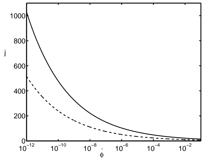
FIG. 3: Numerical results corresponding to the scheme shown in Fig. 2.
