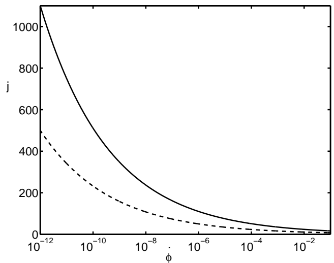
FIG. 2: Analytic results for HAM quantization with l = 3/4 and initial conditions \phi_i = 0 and \dot{\phi}_i > 0 . The solid line corresponds to the case where the turning point of the inflaton is at \phi = 3l_{\text{Pl}} . Sufficient inflation to solve the horizon problem arises in the region above this line. The kinetic bound is satisfied in the region below the dashed line. The two regions do not overlap.
