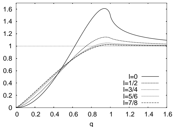
FIG. 8: The behavior of the function D_l for different values of l .
