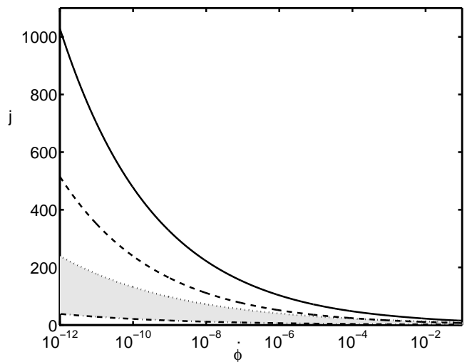
FIG. 6: Numerical results for HAM quantization with l = 3/4 , where the initial value of the inflaton is determined by imposing the uncertainty principle (27). The horizon problem is solved in regions above the solid line and below the dotted line. The region below the dashed line satisfies the kinetic bound. The potential energy of the field exceeds the Planck scale below the dot-dashed line. Successful inflation is possible in the shaded region.
