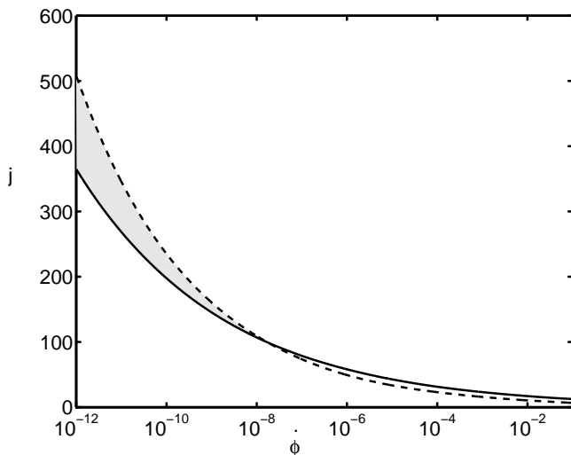
FIG. 5: Numerical results corresponding to the scheme shown in Fig 4.
