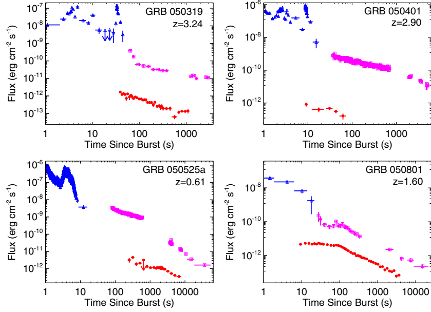
Figure 1. Multi-wavelength light curves for four bursts. The BAT data (blue triangles) have been extrapolated to the X-ray regime as described in Section 3.2. The XRT data are shown with magenta squares, and the ROTSE-III data with red circles. In all cases, the optical flux is below the X-ray flux. The time axis has been corrected for cosmological time dilation. GRB 050319 : the optical data do not show a deviation from a simple power law, while the X-ray data show the typical steep–flat evolution. GRB 050401 : neither the optical nor the X-ray data show deviations from simple power laws. GRB 050525a : the optical light curve shows a steepening at \sim 2000 s, while the X-ray light curve shows a slightly more complicated evolution. GRB 050801 : the optical light curve shows a steepening at \sim 100 s, and the X-ray light curve shows a very similar morphology.
