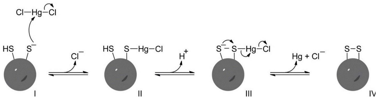
Figure A.3. Oxidation by \text{HgCl}_2 of two closely spaced cysteine sulfur atoms to form a disulfide
