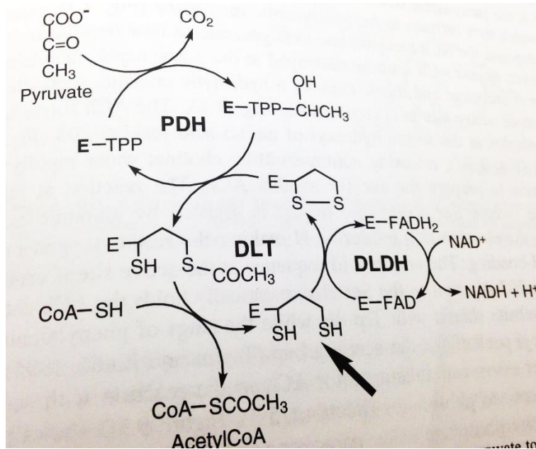
Figure A.2. Inactivation of DHL enzyme by \text{As}^{3+} (Crosby 1998).
