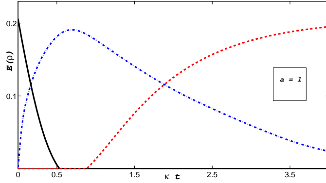
FIG. 7. Entanglement monotone is plotted for cavity-cavity (solid line), reservoir-reservoir (dashed line), and four qubits (dashed-dotted line) for states (18) for a = 1 .
