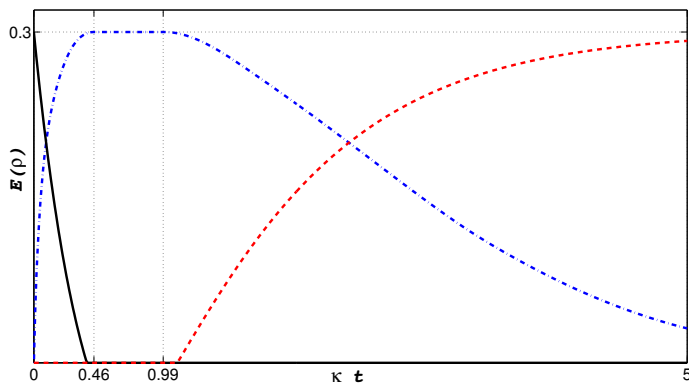
FIG. 3. E -monotone is plotted against parameter \kappa t for cavity-cavity qubits (black solid line), reservoir-reservoir qubits (red dashed line) and all four qubits (blue dashed-dotted line). In the time window when there is no entanglement between cavity qubits and reservoir qubits, the multipartite entanglement exhibits an abrupt change to a value that remains constant in that window.
