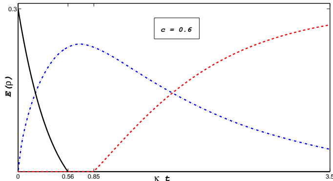
FIG. 9. Entanglement monotone is plotted for cavity-cavity (solid line), reservoir-reservoir (dashed line), and four qubits (dashed-dotted line) for states (21) for c = 0.6 .
