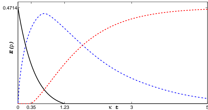
FIG. 2. E -monotone is plotted against parameter \kappa t for cavity-cavity qubits (black solid line), reservoir-reservoir qubits (red dashed line) and all four qubits (blue dashed-dotted line) for \alpha = \sqrt{1/3} and \beta = \sqrt{2/3} .
