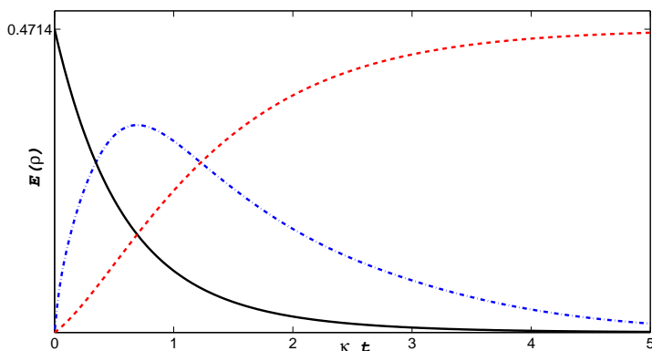
FIG. 1. E -monotone is plotted against parameter \kappa t for cavity-cavity qubits (black solid line), reservoir-reservoir qubits (red dashed line) and all four qubits (blue dashed-dotted line) for \alpha = \sqrt{2/3} and \beta = \sqrt{1/3} . See text for more description.
