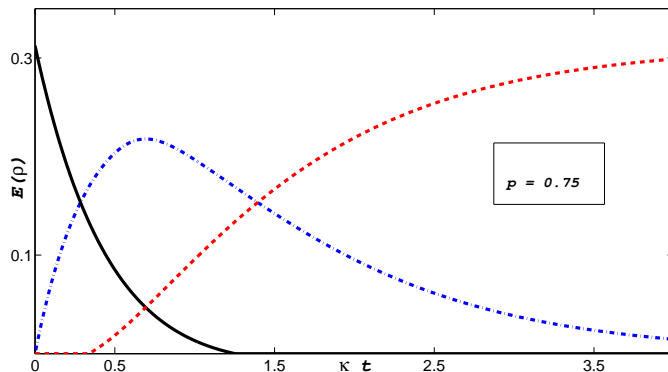
FIG. 6. Same caption as Figure (5) but for p = 0.75 .
