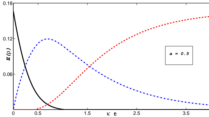
FIG. 8. Same caption as Figure 7 but for a = 0.5 .
