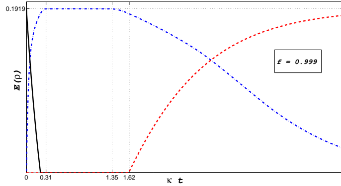
FIG. 11. Entanglement monotone is plotted for cavity-cavity (solid line), reservoir-reservoir (dashed line), and four qubits (dashed-dotted line) for states (Eq. 24) for f = 0.999 .
