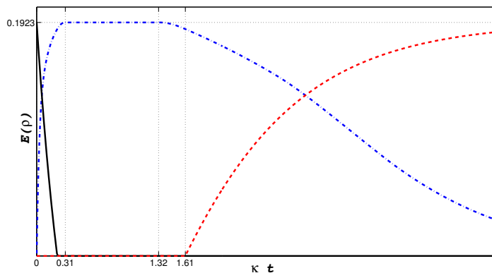
FIG. 4. Same caption as Figure (3). See the text for more descriptions.
