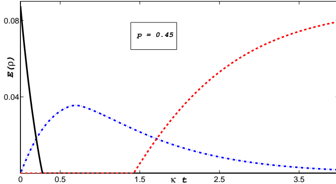
FIG. 5. Entanglement monotone for cavity qubits (solid line), reservoir qubits (dashed line), and collective state of four qubits (dashed-dotted line) is plotted against parameter \kappa t for Werner states with p = 0.45 .
