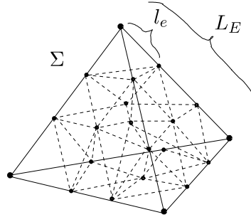
Figure 3. A tetrahedron \Sigma subdivided into smaller tetrahedra \sigma . The length L_E of a coarse edge E is the sum of all the lengths l_e of edges e \subset E that constitute E .
