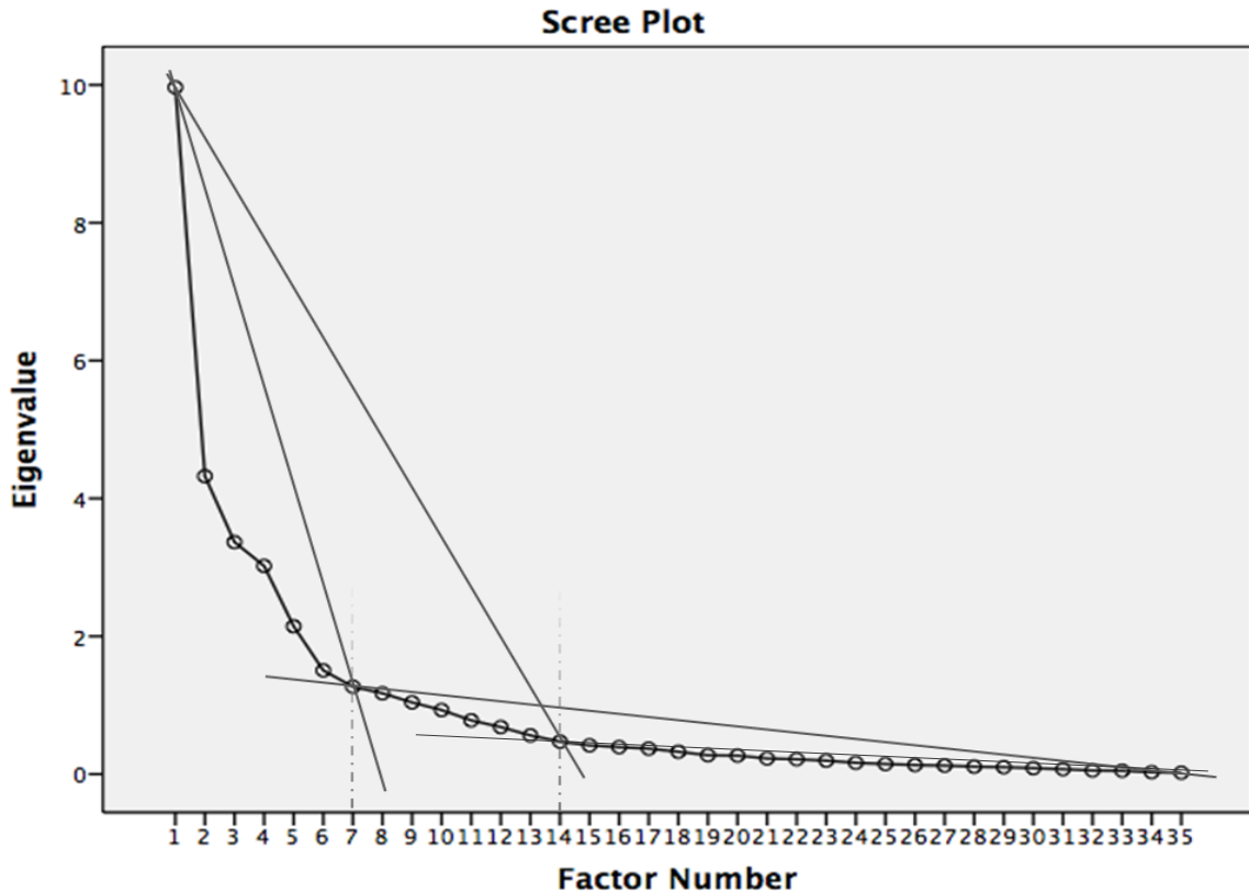
Figure 11: Scree Test
