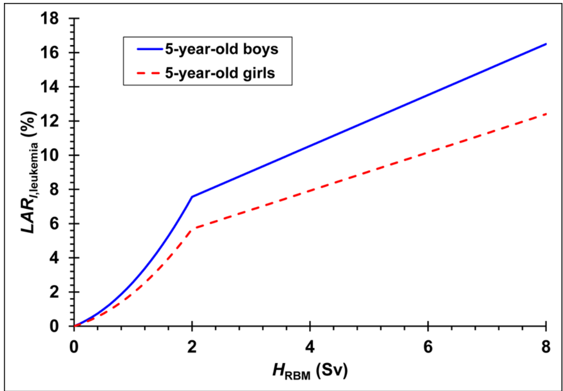
Figure 1. LAR of leukemia incidence for 5-year old boys (solid line) and a 5-year-old girls (dashed line) calculated by our model as a function of the mean equivalent dose in the red bone marrow.
