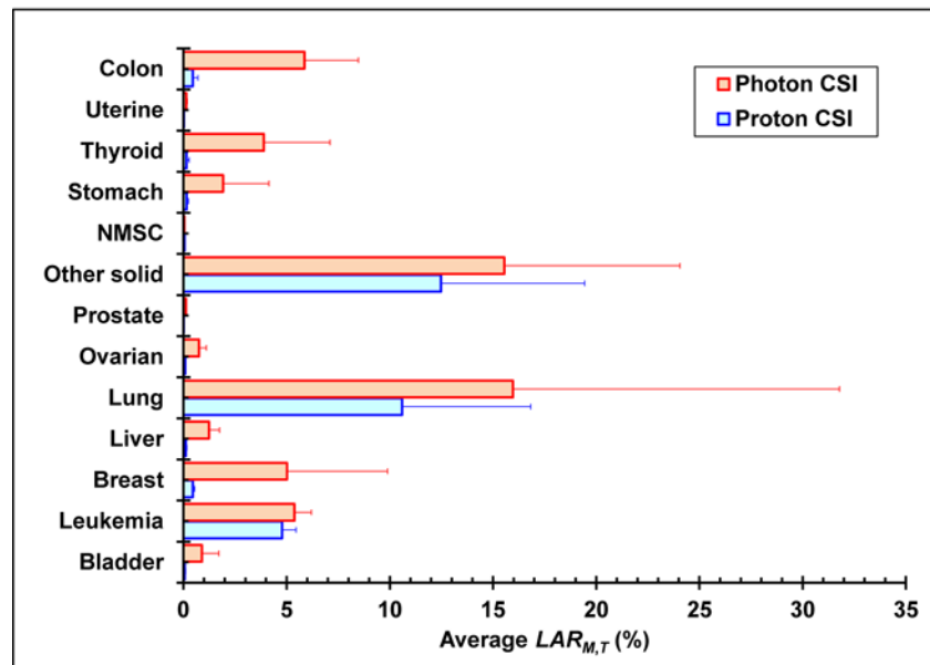
Figure 2. Mean LAR values of SMN incidence (top panel) and mortality (bottom panel), averaged across all patients for photon CSI and proton CSI. One-sided error bars represent the 95% confidence interval in each mean value for a particular SMN and do not take into account the large uncertainties in the risk model.
