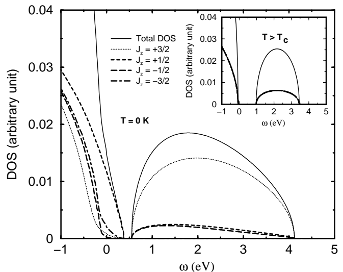
FIG. 2: Decomposition of the density-of-states in terms of J_z components, for J_c = 3.0 eV at T = 0 (main panel) and T > T_c (inset). The chiral nature of the holes due to spin-orbit coupling mixes up states with different J_z components, making the total DOS only partially polarized at T = 0 .
