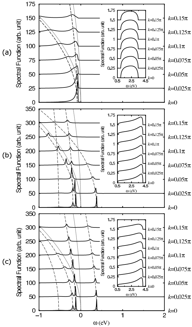
FIG. 3: Spectral functions near the center of the Brillouin zone for J_c = 3.0 eV at (a) T > T_c along any direction, (b) T = 0 along the direction parallel and (c) perpendicular to the magnetization. Insets display a zoom of the impurity band region. Each spectral curve corresponds to a different value of the magnitude of the momentum k , as indicated at the right of the graphs, and the baseline of each spectrum is shifted proportionally to k for clarity. In the main panels the dashed curves represent the renormalized valence bands. For comparison, the valence bands of pure GaAs are also displayed (dotted curves). The scale in the insets is blown-up by a factor of 100 in (a) and 200 in (b) and (c).
