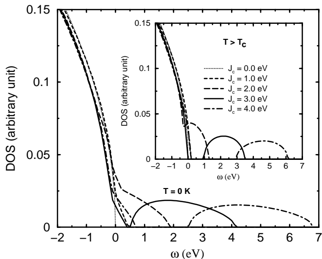
FIG. 1: Density-of-states for J_c = 1.0, 2.0, 3.0, and 4.0 eV, at T = 0 (main panel) and T > T_c (inset). The appearance of an impurity band is evident for J_c > 2.0 eV. The broader impurity band at T = 0 , compared to that at T > T_c , indicates that lifetime of the bound-state holes decreases as the system becomes magnetically ordered.
