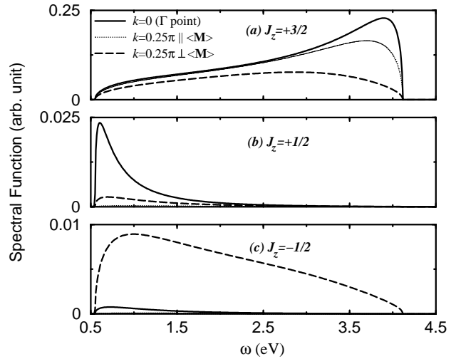
FIG. 4: Variation of the J_z components of the impurity band spectral function for J_c = 3.0 eV and T = 0 ((a) J_z = +3/2 , (b) J_z = +1/2 , and (c) J_z = -1/2 ) as the magnitude of the momentum k changes from 0 (solid curve) to k = 0.25\pi along the direction parallel (dotted curve) and perpendicular (long-dashed curve) to the average magnetization. Notice that the three graphs have different scales.
