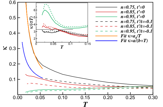
FIG. 15: (Color online) Thermal conductivity versus temperature for U = 6t , N_c = 16 , and 4t = 1 . Inset: Wiedemann Franz ratio for the same physical parameters. The horizontal solid line labels the constant \pi^2/3 .
