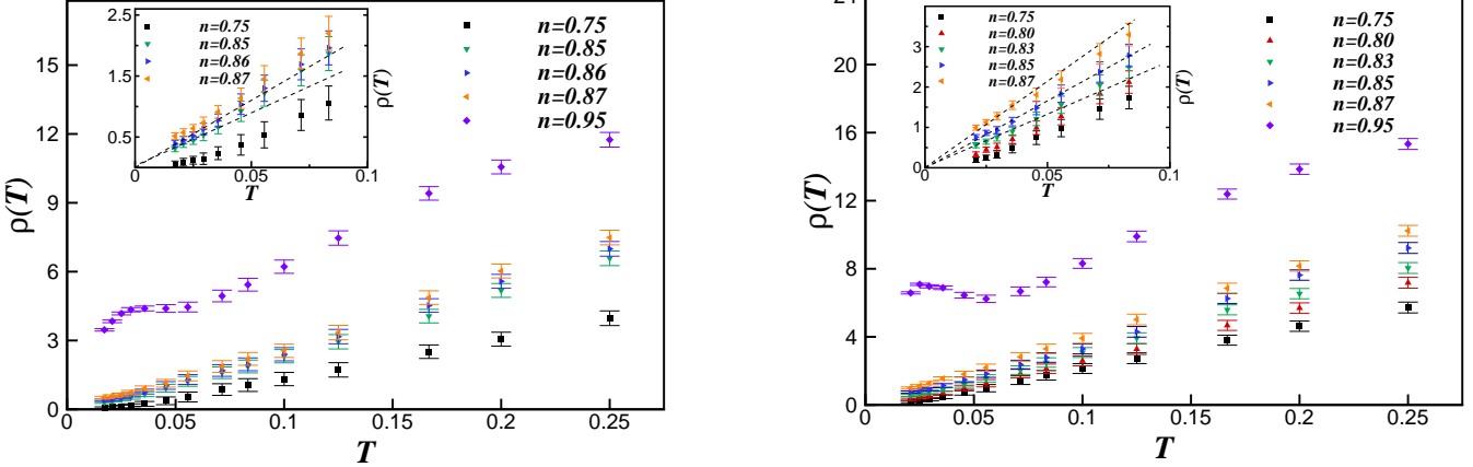
FIG. 14: (Color online) Resistivity versus temperature for t' = 0 (left) and t'/t = -0.1 (right) with U = 6t , N_c = 16 , and 4t = 1 . The dashed lines in the insets are linear fits. For t' = 0 , the resistivity shows linear- T behavior for n = 0.85 and n = 0.86 . For t'/t = -0.1 , the resistivity shows linear- T behavior from n = 0.83 to n = 0.87 .
