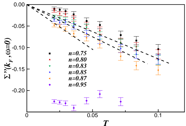
FIG. 10: (Color online) Temperature dependence of the imaginary part of the self energy \Sigma''(\mathbf{k}_F, \omega = 0) at the Fermi energy and momenta, U = 6t , N_c = 16 , 4t = 1 , and t'/t = -0.1 . The self energy for filling between n = 0.83 and 0.87 shows a linear- T behavior.
