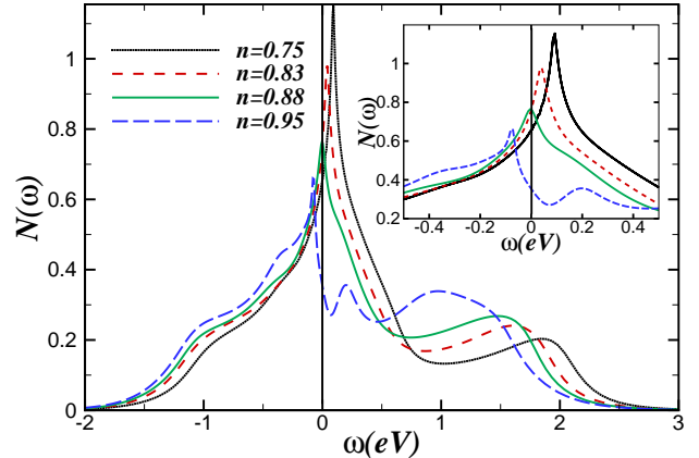
FIG. 5: (Color online) The single-particle density of states for t' = 0 , U = 6t , 4t = 1 , N_c = 16 and \beta = 58 . The density of states shows low-energy particle-hole symmetry at the filling of n = 0.88 .
