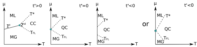
FIG. 17: Schematic chemical potential-temperature ( \mu - T ) phase diagram for three values of t' : (from left to right) t' > 0 , t' = 0 , t' < 0 scenario presented in this paper and a t' < 0 scenario based on a Lifshitz transition. CC (QC) indicates the classical (quantum) critical region. ML (MG) indicates the Mott liquid (gas) region. T^* is the crossover temperature between the Mott liquid and the critical region, T_{FL} separates the Mott gas from the critical region. Note here, we have ignored other phases to focus attention on the quantum critical region.
