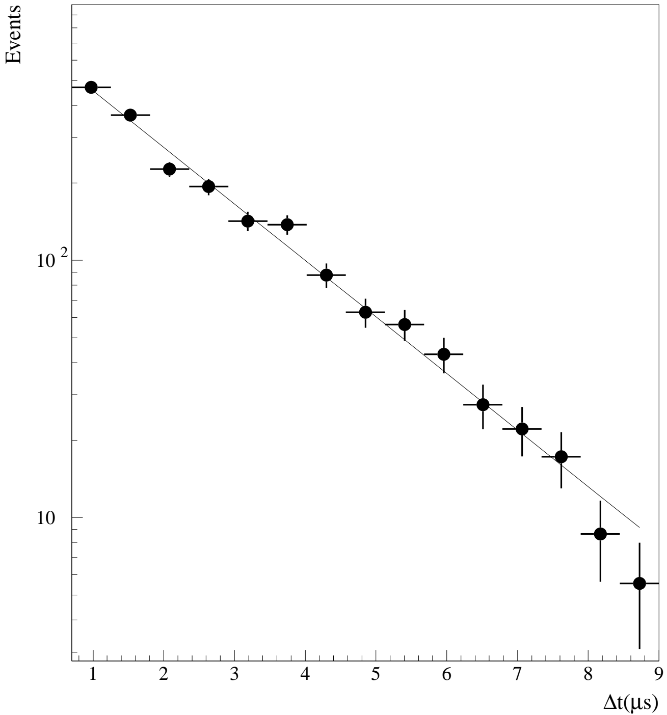
FIG. 8. The distribution of time \Delta t_{\mu e} between the \mu^- and the decay e^- in the inclusive sample, ^{12}\text{C}(\nu_{\mu}, \mu^-)\text{X} . The best fit (solid line) curve corresponds to a lifetime of 1.98 \pm 0.06 \mu\text{s} .
