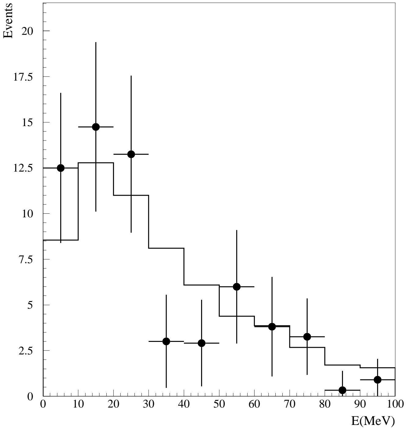
FIG. 16. The observed and expected (solid line) \mu^- kinetic energy distribution for beam excess-events in the ^{12}\text{C}(\nu_{\mu}, \mu^-)^{12}\text{N}_{g.s.} sample.
