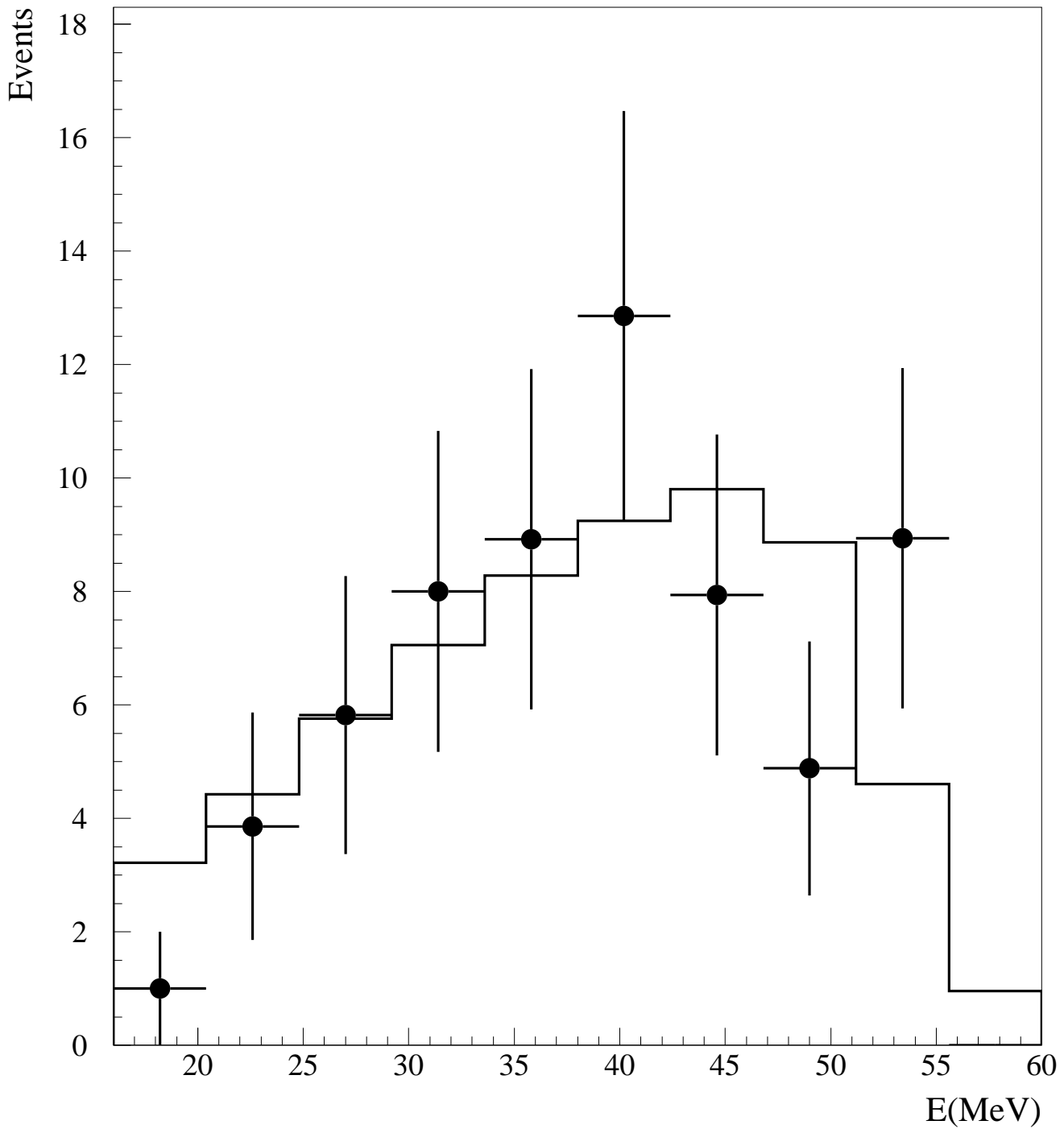
FIG. 14. The observed and expected (solid line) e^- energy distribution for beam-excess events in the ^{12}\text{C}(\nu_\mu, \mu^-)^{12}\text{N}_{g.s.} sample. The expected distribution was obtained from a large sample of stopping cosmic ray events.
