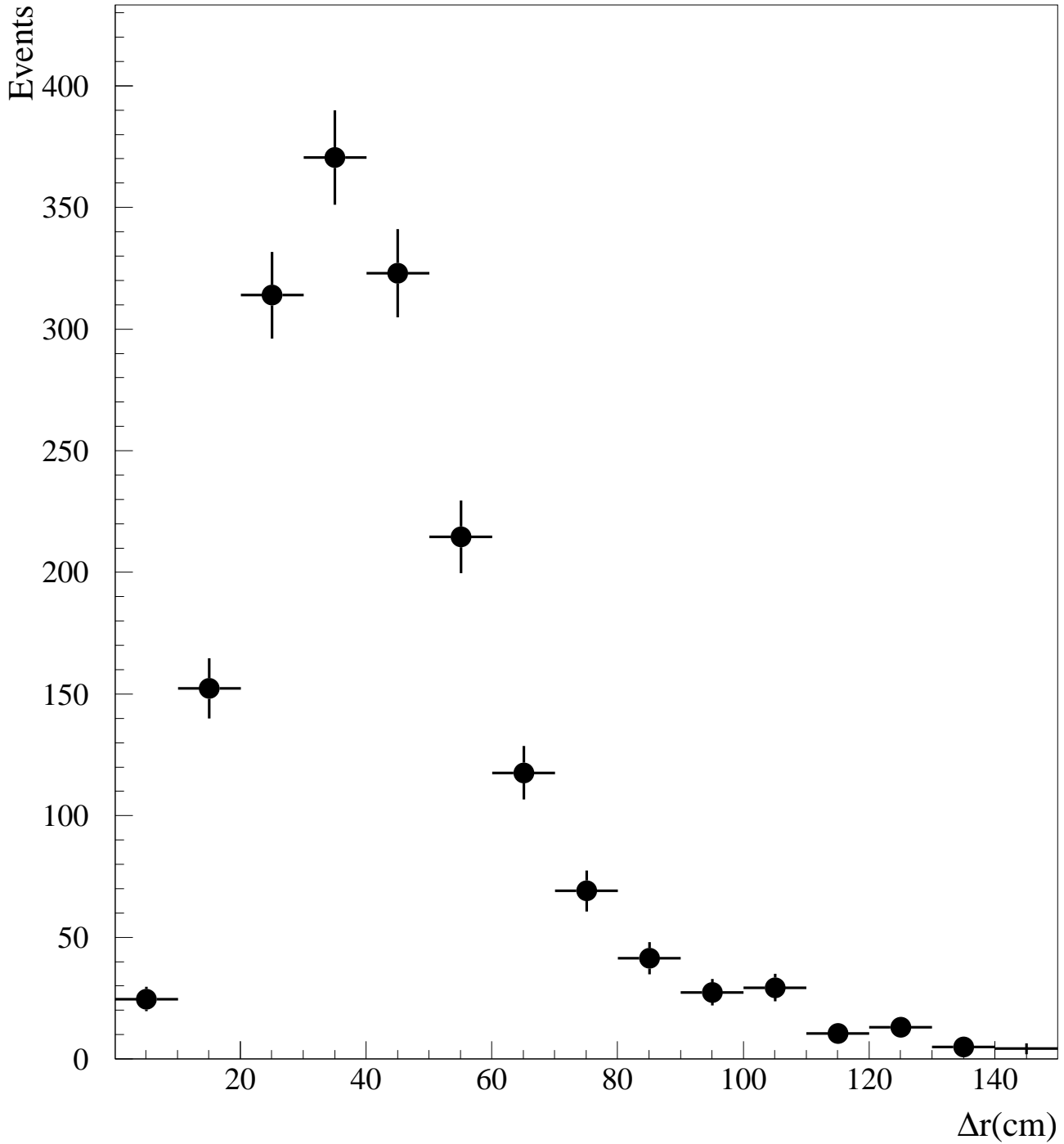
FIG. 9. The distribution of the distance between the reconstructed position of the \mu^- and the e^- in the beam-excess inclusive sample, ^{12}\text{C}(\nu_\mu, \mu^-)\text{X} .
