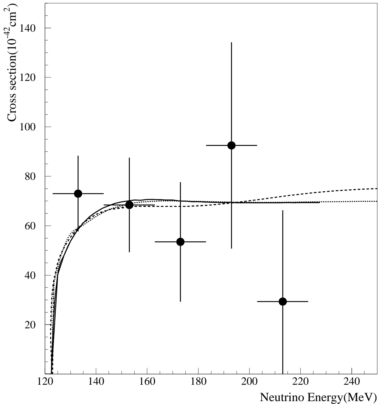
FIG. 17. The measured cross section for the process ^{12}\text{C}(\nu_{\mu}, \mu^{-})^{12}\text{N}_{g.s.} compared with three theoretical calculations obtained from Ref. 20.
