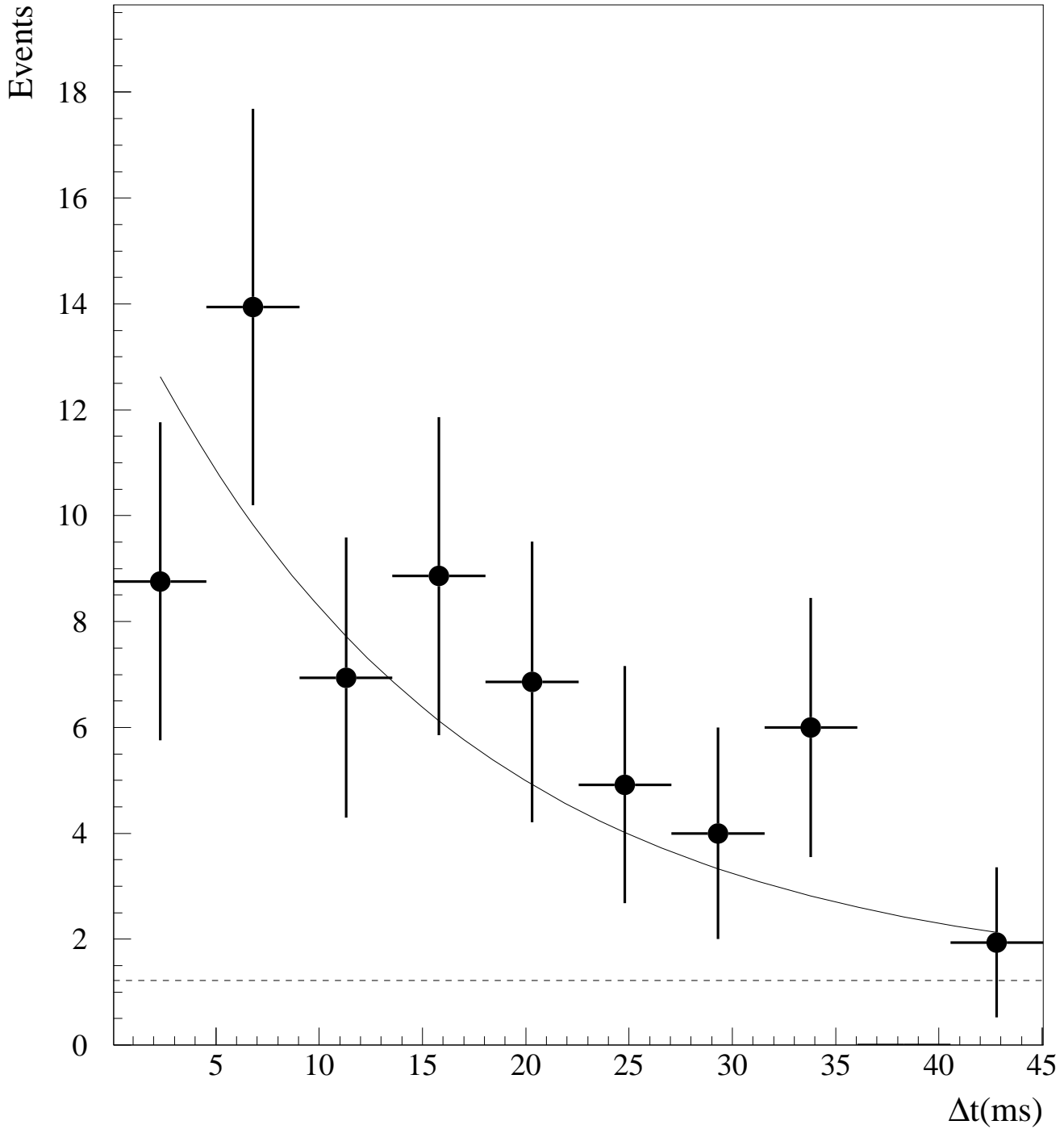
FIG. 11. The distribution of time between the e^- and e^+ for beam-excess events in the ^{12}\text{C}(\nu_{\mu}, \mu^-)^{12}\text{N}_{g.s.} sample. The expected distribution is shown with the solid line. The calculated accidental contribution is shown by the dashed line.
