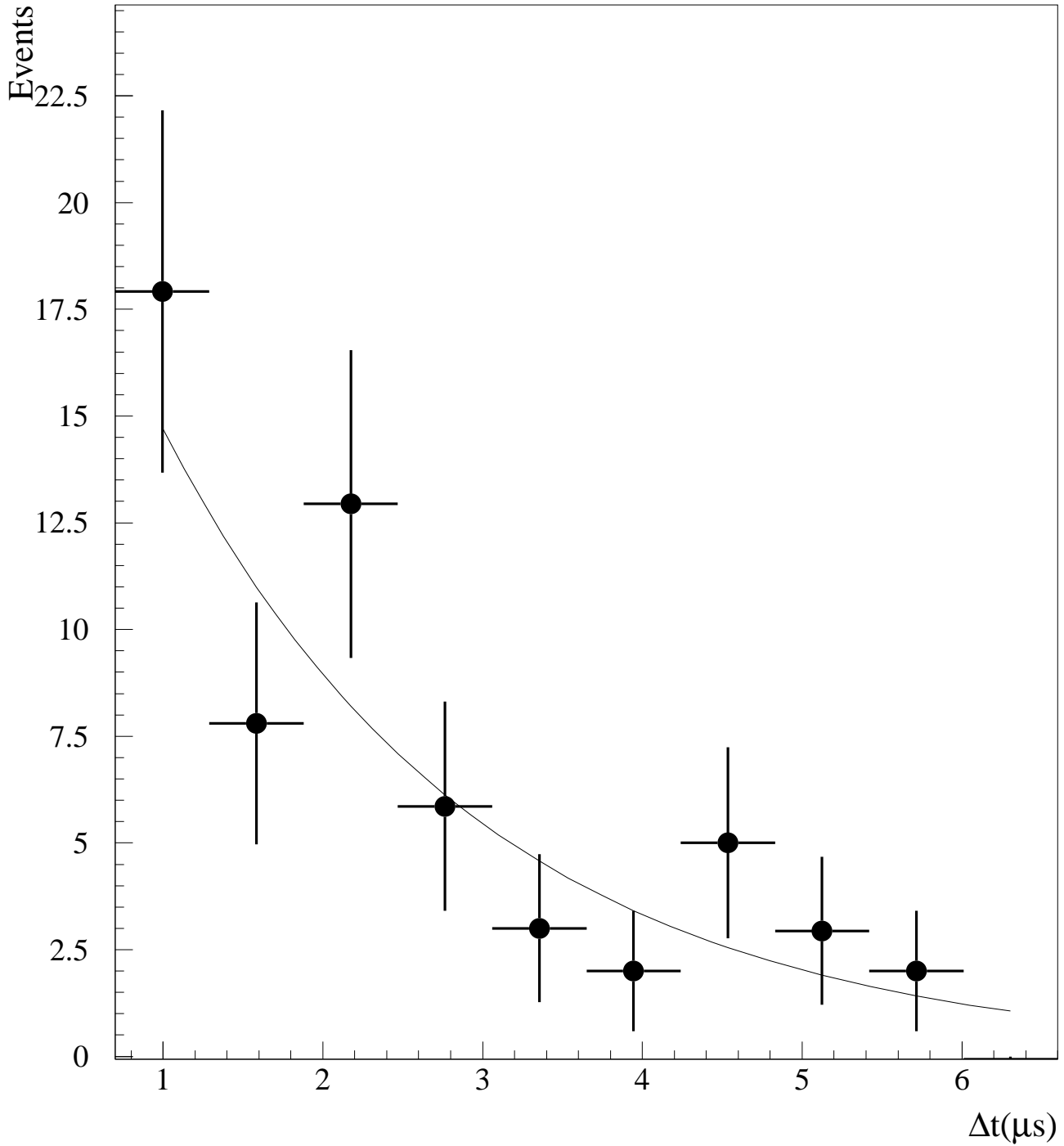
FIG. 15. The obtained and expected (solid line) distribution of time between the \mu^- and the subsequent decay e^- for beam-excess events in the ^{12}\text{C}(\nu_{\mu}, \mu^-)^{12}\text{N}_{g.s.} sample.
