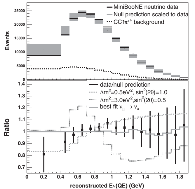
FIG. 1. The top plot shows the E_\nu^{\text{QE}} distribution for neutrino data (black) with statistical error rectangles (thickness of line indicates size of statistical error), and the prediction assuming no oscillations [area normalized to number of data events (grey)]. Attached to the prediction are the diagonal elements of the shape error matrix. The predicted CC1 \pi background (dashed line) events are also shown. The background antineutrino events are negligible. The bottom plot shows the ratio of data to no oscillations (black solid line), and the ratio of no oscillations to \Delta m^2 = 0.5 eV 2 , \sin^2 2\theta = 1.0 disappearance (dashed line), \Delta m^2 = 3.0 eV 2 , \sin^2 2\theta = 0.5 disappearance (dotted line), and for the minimum \chi^2 = 12.72 (13 DF) at \Delta m^2 = 17.5 eV 2 , \sin^2 2\theta = 0.16 (solid grey line).
