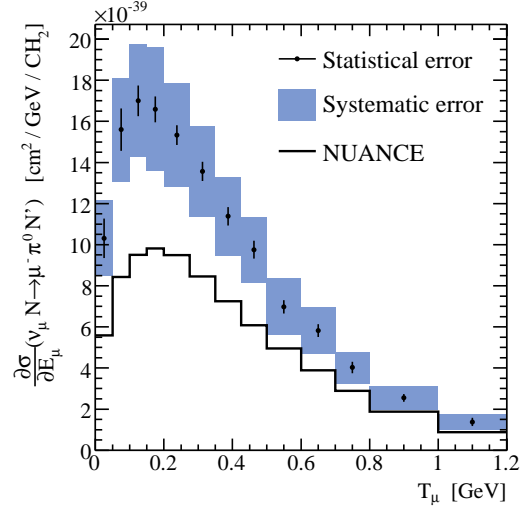
FIG. 10. (color online) The flux-averaged ( 0.5 < E_\nu < 2.0 GeV) differential cross section in E_\mu with total systematic uncertainty of 15.8%. The central-value measurement, uncertainties, and correlation matrix are tabulated in Table VIII of the appendix.
