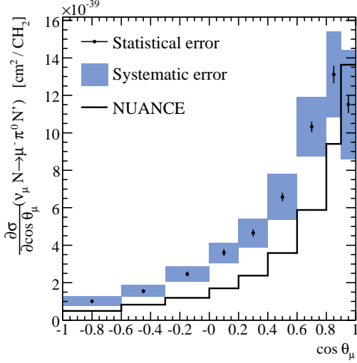
FIG. 11. (color online) The flux-averaged ( 0.5 < E_\nu < 2.0 GeV) differential cross section in \cos \theta_\mu with total systematic uncertainty of 17.4%. The central-value measurement, uncertainties, and correlation matrix are tabulated in Table IX of the appendix.
