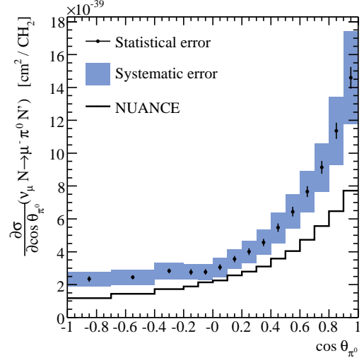
FIG. 13. (color online) The flux-averaged ( 0.5 < E_\nu < 2.0 GeV) differential cross section in \cos \theta_{\pi^0} with total systematic uncertainty of 16.3%. The central-value measurement, uncertainties, and correlation matrix are tabulated in Table XI of the appendix.
