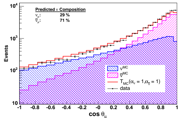
FIG. 5: (Color online) The \cos \theta_\mu distribution of the CCQE sample by neutrino type before fitting. As printed on the figure, 29% of the sample is predicted to be induced by neutrinos. The Monte Carlo sample has been normalized to 5.66 \times 10^{20} protons on target.
