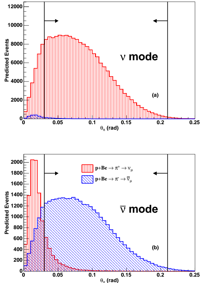
FIG. 1: (Color online) Predicted angular distributions of pions with respect to the incident proton beam ( \theta_\pi ) producing \nu_\mu and \bar{\nu}_\mu in (a) neutrino mode and (b) anti-neutrino mode. Only pions leading to \nu_\mu and \bar{\nu}_\mu events in the detector are shown, and all distributions are normalized to 5.66 \times 10^{20} protons on target. Arrows indicate the region where HARP data [14] are available.
