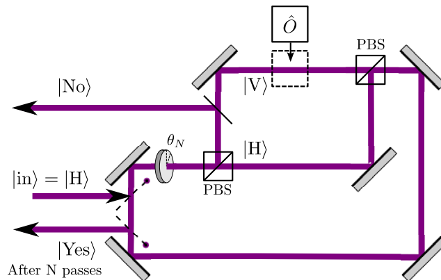
Figure 2. IQT apparatus based on an N -pass IFM in the polarization interferometer. With each pass, the photon's polarization is rotated by an angle \theta_N . The presence of an object prevents accumulation of polarization rotation and is similar to the quantum Zeno effect [4, 5]. An additional beam splitter inside the polarization interferometer models unavoidable loss in the arm accessible by the object as well as controlled loss that is adjusted to provide the best performance of the IQT apparatus.
