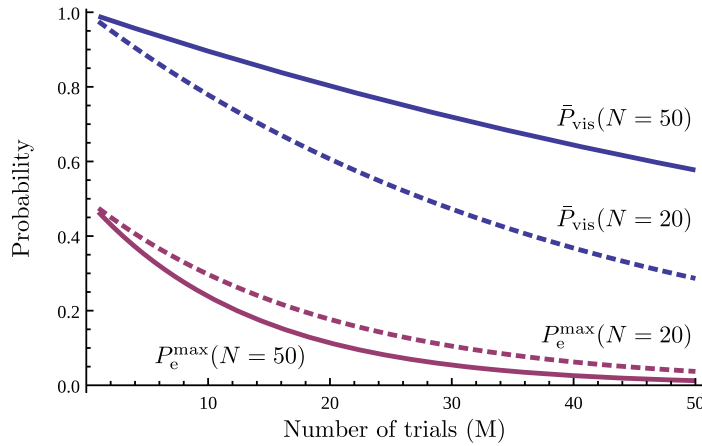
Figure 5. The probability of the tripwire being invisible \bar{P}_{\text{vis}} and the maximum error bound P_e^{\text{max}} are given as functions of the number of trials M , for a given number of passes N = 20 and N = 50 . As N gets larger, \bar{P}_{\text{vis}} will stay closer to one, while P_e^{\text{max}} will go faster to zero.
