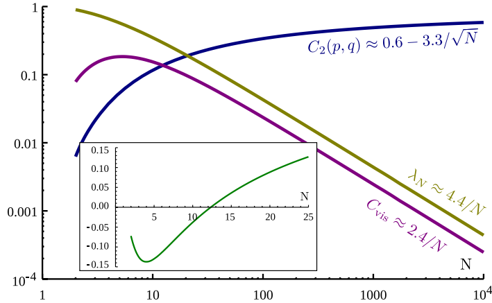
Figure 4. The Chernoff C_2(p, q) and visibility C_{\text{vis}} distances as a function of the number of passes N as well as the amount of loss, \lambda_N , in the detection arm required for partial Zeno to take place. The inset shows a difference between those distances. Invisible detection becomes possible when this difference becomes positive.
