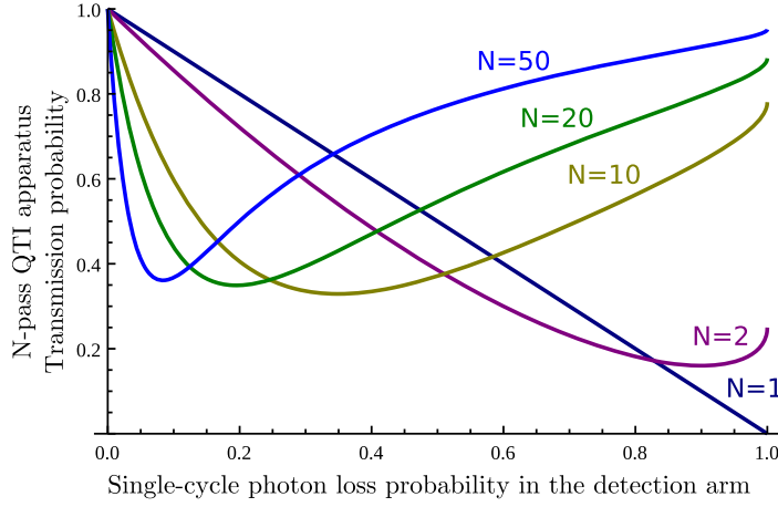
Figure 3. The single-photon transmission probability in an N -pass IQT apparatus P_{\text{tr}} for N\theta_N = \pi/2 as a function of single-cycle probability of photon loss in the detection arm. Loss in an N -pass IQT is optimized for this partial Zeno effect to take place. The detection of an object is based on increase of transmission.
