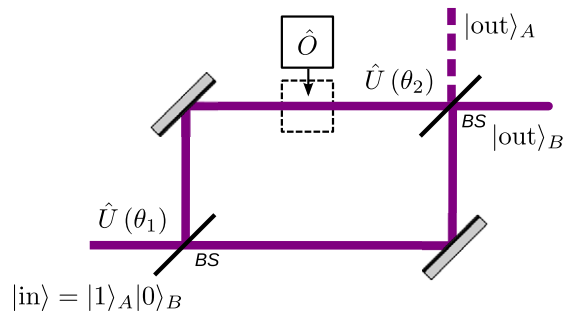
Figure 1. A lossless MZI in a dark port arrangement, \theta_1 + \theta_2 = \pi/2 , and in a zero phase difference between its arms constitutes a simple IFM setup with efficiency \eta \leq 1/2 . This scheme allows for interaction-free hypothesis testing of a path being blocked ( h_1 ) or clear ( h_0 ).
