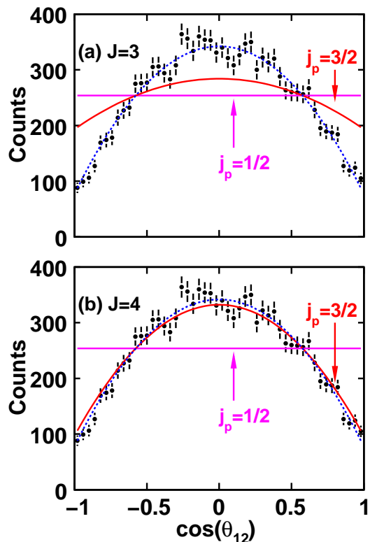
FIG. 13. (Color online) Angular correlations for the 5.93-MeV state of {}^8\text{B} . Events were selected using both the G4 and G6 gates in Fig. 11. The angle \theta_{12} in the relative angle between the initial proton decay axis and the subsequent {}^3\text{He}+\alpha decay axis in the {}^8\text{B} center-of-mass frame. The proton and \alpha particle are emitted in the same direction when \theta_{12}=0 . The solid curves are predictions for pure values of j_p , while the dashed curves are for mixed values where the degree of mixing was chosen to best fit the data.
