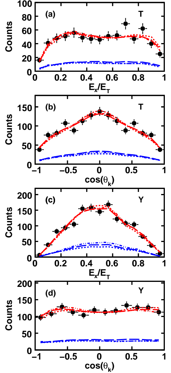
FIG. 6. (Color online) Projected correlations in (a,b) “T” and (c,d) “Y” Jacobi systems for the three-body decay of {}^6\text{Be} formed in the second step of {}^8\text{C}_{g.s.} decay. Angular correlations are shown in (b) and (d) and energy correlations are shown in (a) and (c). The data points are the experimental data, while simulated results are indicated by the curves which pass through the data points. The lower curves are estimates of the “backgrounds” of incorrectly identified events. The short and long-dashed and solid curves are associated with simulations (A), (B), and (C), respectively (see text).
