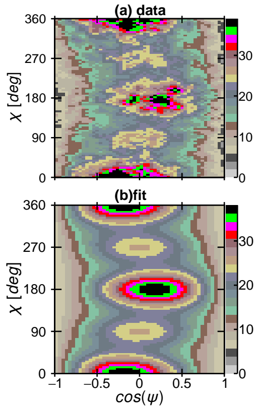
FIG. 9. (Color online) \cos\psi - \chi angular correlation plots obtained for the s^* = 3^+ excited state in {}^6\text{Li} with \theta_{lab}^* > 2^\circ . (a) efficiency-corrected experimental data. (b) fitted correlation using Eq. (15).
