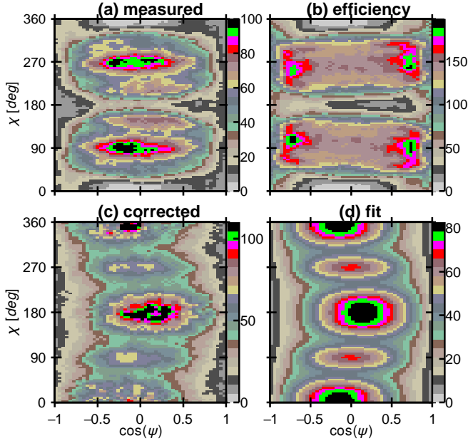
FIG. 3. (Color online) \cos \psi - \chi angular correlation plots obtained for the s^* = 7/2^- excited state in {}^7\text{Be} with \theta_{lab}^* > 2^\circ . (a) directly measured raw angular correlations without corrections, (b) Simulated detector efficiency, (c) measured correlations corrected for the detected efficiency (d) fitted correlation using Eq. (15).
