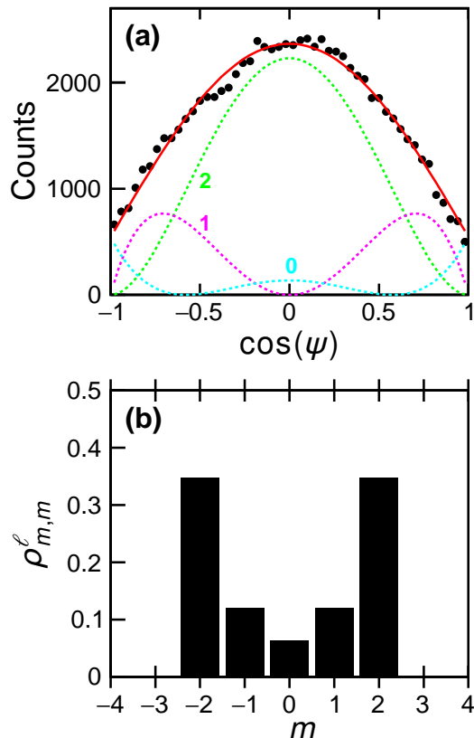
FIG. 10. (Color online) (a) The efficiency-corrected correlation plot for the s^*=3^+ excited state of {}^6\text{Li} projected on the \cos\psi axis. (b) Probability distribution of the projection m of the decay orbital angular momentum. In (a), the solid curve show a fit with the individual m components indicated by the dashed curves.
