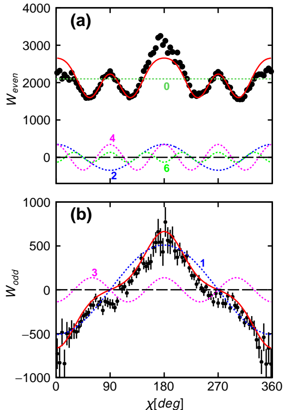
FIG. 5. (Color online) Projected (a) W_{even} and (b) W_{odd} correlation distributions for the s^*=7/2^- excited state of {}^7\text{Be} . The solid curves show fits with Eqs. (18) and (20) while the dashed curves give individual \cos m\chi components where each curve is labeled by the value of m .
