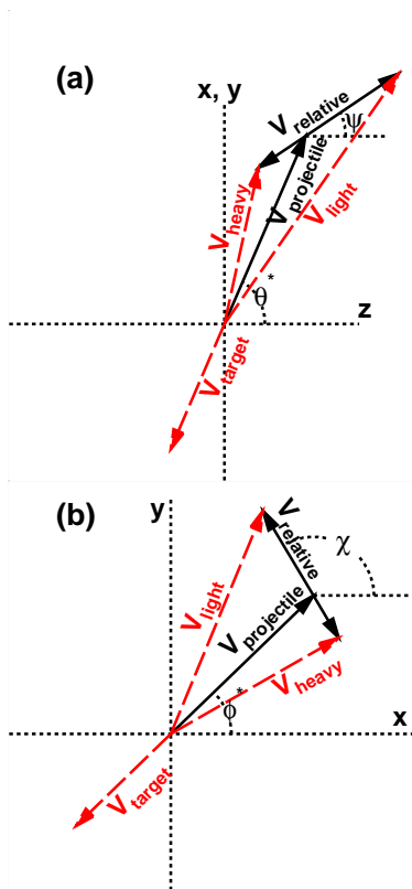
FIG. 1. (Color online) Schematic showing the definition of the angles \theta^* , \phi^* , \psi , and \chi in terms of the reaction-center-of-mass velocity vectors of the projectile ( V_{\text{projectile}} ) and target ( V_{\text{target}} ) nuclei and those of the light ( V_{\text{light}} ) and heavy ( V_{\text{heavy}} ) decay products of the projectile. The experimental angular correlations were analyzed with the z axis aligned along the beam axis and the x axis in the reaction plane.
