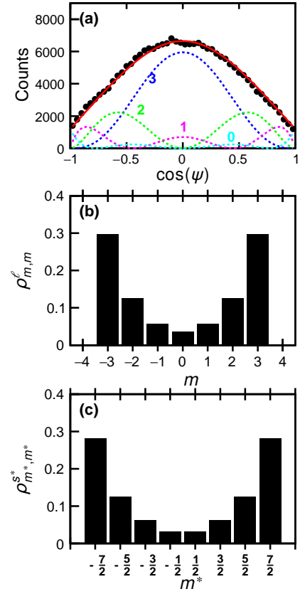
FIG. 4. (Color online) (a) The efficiency-corrected correlation plot for the s^* = 7/2^- excited state of {}^7\text{Be} projected on the \cos \psi axis. (b) Probability distribution for the projection m of the decay orbital angular momentum. (c) Probability distribution for the projection m^* of the {}^7\text{Be} spin. In (a), the solid curve shows a fit with the individual m components indicated by the dashed curves.
