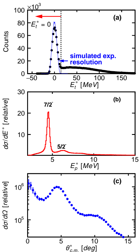
FIG. 2. (Color online) (a) Experimental distribution of the excitation energy of the {}^9\text{Be} target nucleus deduced from detected {}^3\text{He}+\alpha events obtained with the {}^7\text{Be} beam. (b) Distribution of {}^7\text{Be} projectile excitation energy associated with detected events where the target remained in its ground state [ E_t^*=0 ]. (c) Angular distribution of the scattered projectile in the reaction center-of-mass frame for the E^*=4.57\text{-MeV} , s^*=7/2^- excited state of {}^7\text{Be} with E_t^*=0 .
