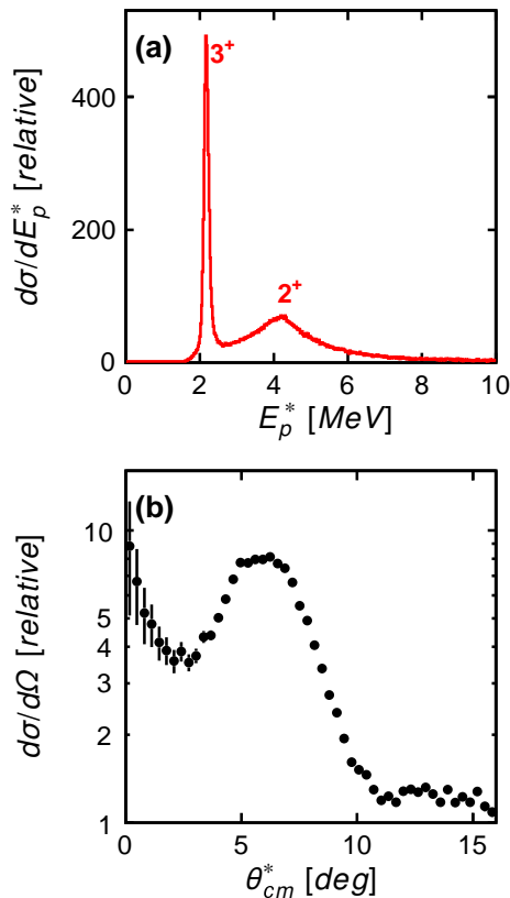
FIG. 8. (Color online) (a) Efficiency-corrected projectile excitation-energy distribution determined from detected d + \alpha events for E_t^* = 0 with the {}^6\text{Li} beam. (b) Angular distribution of the scattered projectile extracted for the s^* = 3^+ level.
