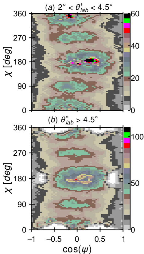
FIG. 6. (Color online) Efficiency-corrected correlation plots for the s^*=7/2^- excited state of {}^7\text{Be} for the two indicated gates on the projectile scattering angle \theta^* .
