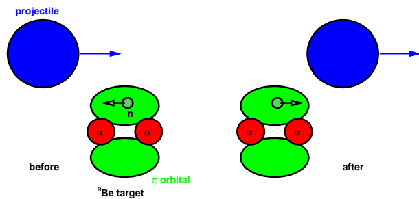
FIG. 12. (Color online) Schematic illustrating the suggested orientation of the target nucleus for the inelastic interactions considered in this work. The ground-state of {}^9\text{Be} target nucleus is depicted as two alpha particles plus a valence neutron in a \pi molecular orbit. The total angular momentum of the valence neutron is flipped due to interactions with the projectile.
