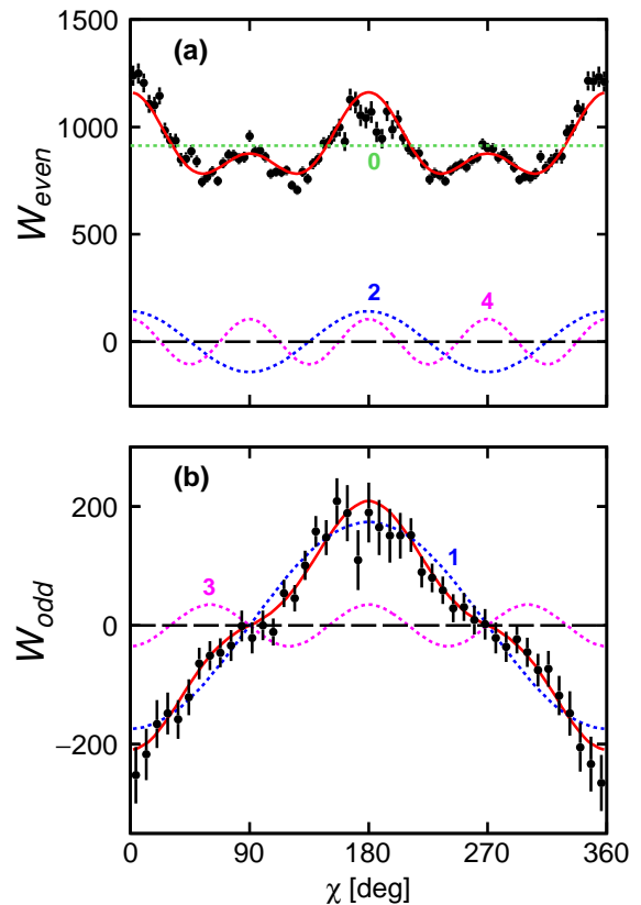
FIG. 11. (Color online) As in Fig. 5, but for the s^*=3^+ excited state of {}^6\text{Li} .
