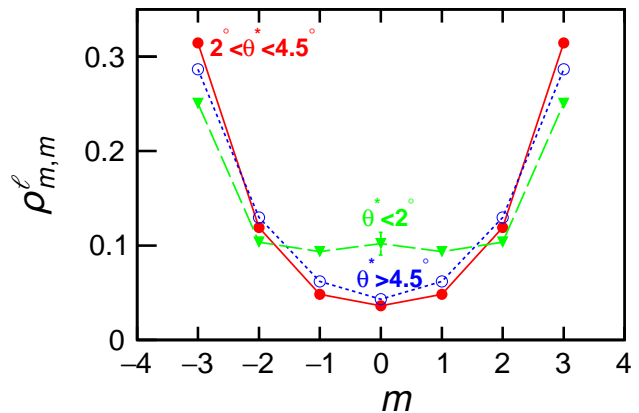
FIG. 7. (Color online) Probability distribution of the projection m of the decay orbital angular momentum for three regions of laboratory scattering angle obtained for the s^*=7/2^- excited state of {}^7\text{Be} .
