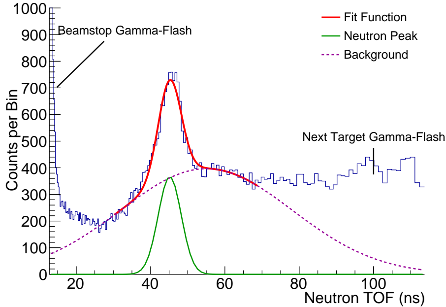
Fig. 4. Neutron time-of-flight spectrum for the ^{12}\text{C}(d,n)^{13}\text{N} reaction at \theta_{CM} = 12^\circ ( \theta_{lab} = 144^\circ ), in inverse kinematics, with a beam energy of E_{^{12}\text{C}} = 41.7 MeV. The gaussian fit to the peak for population of the ground state, the background, and the sum fit function are shown in green, magenta, and red respectively. The timing of the \gamma flash from the next beam pulse is shown.
