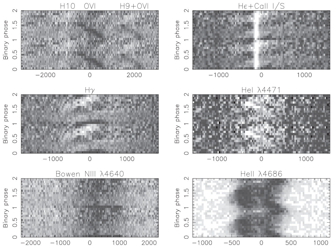
Fig. 2.—Trailed spectrogram of selected lines folded in 13 phase bins. [See the electronic edition of the Journal for a color version of this figure.]
