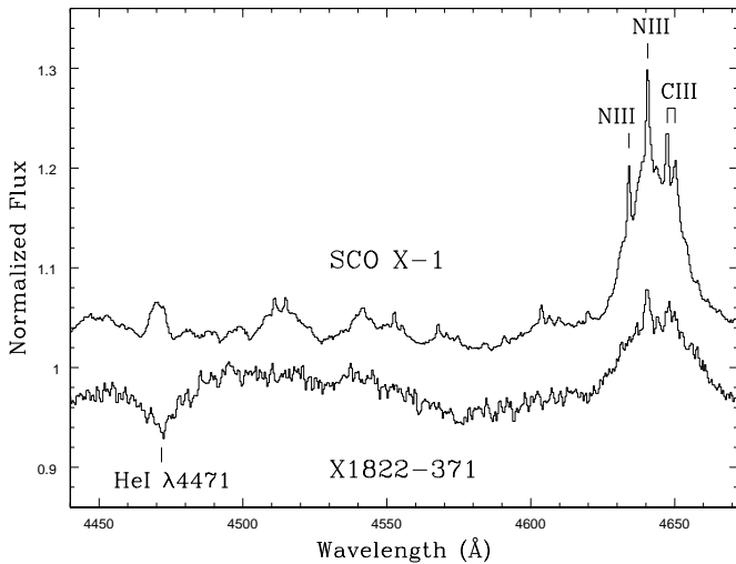
FIG. 6.—Doppler-corrected averaged spectra of Sco X-1 and X1822–371, in the rest frame of the companion. In the latter case we have used \gamma = -43 \text{ km s}^{-1} and K_2 = 300 \text{ km s}^{-1} .
