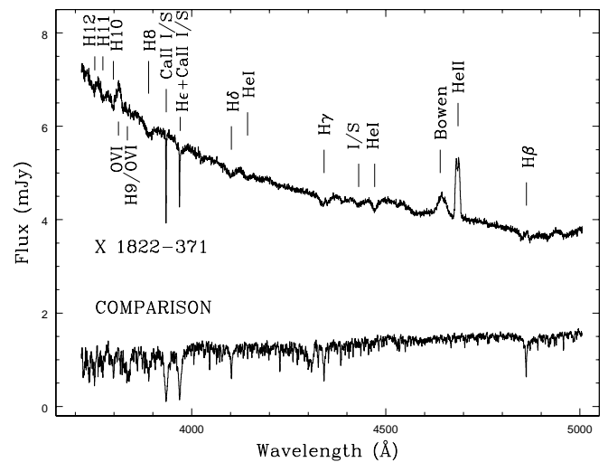
FIG. 1.—Average optical spectrum of X1822–371 and the comparison star in the slit. The main emission and absorption features are indicated.
