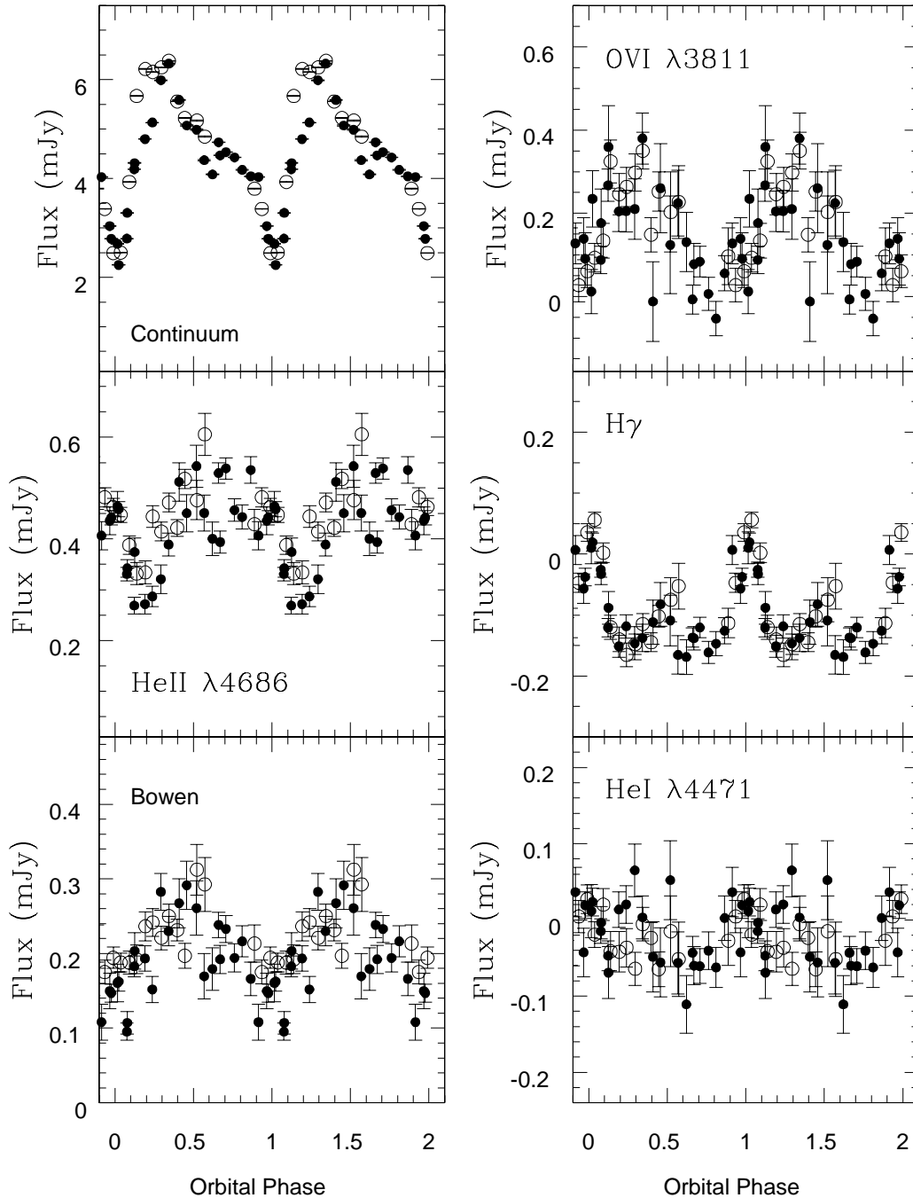
FIG. 4.—Light curves of the continuum (4000–4600 Å) and selected emission/absorption lines. Filled and open circles correspond to the nights of June 10 and 11, respectively.
