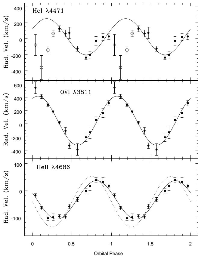
FIG. 3.—Radial velocity curves of He I \lambda 4471 (top), O VI \lambda 3811 (middle), and the wings of He II \lambda 4686 (bottom). The latter was obtained by cross-correlation with a double-Gaussian template of FWHM = 100 km s -1 and separation a = 900 km s -1 (see § 5 for details). Best sine wave fits are shown, after masking a few outliers, marked with open circles, for He I \lambda 4471 (see text for details). The dotted line displays the radial velocity curve of the neutron star, using the pulse-timing ephemeris from JvdK.
