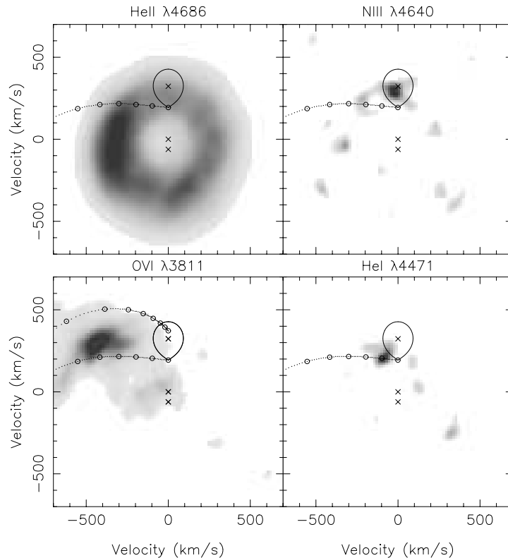
FIG. 5.—Doppler maps of several spectral features. We have overplotted the Roche lobe of the companion star, the gas stream trajectory, and the compact object's position for q = 0.29 , which assumes M_1 = 1.4 M_\odot (i.e., K_2 = 324 \text{ km s}^{-1} ). In the map of O VI we also plot the Keplerian velocity of the disk along the gas stream path. All the images were computed for a systemic velocity \gamma = -43 \text{ km s}^{-1} . [See the electronic edition of the Journal for a color version of this figure.]
