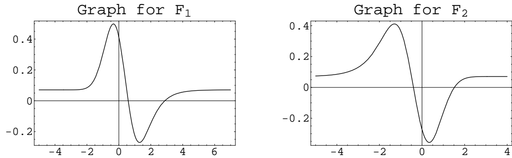
Figure 4.1: Parameter values: \alpha = 1, \lambda = 0.1 .
