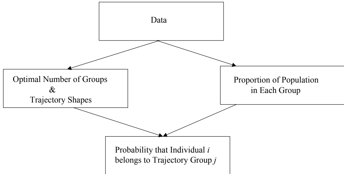
Figure 3.2 : An Overview of Nagin (1999)'s Model
