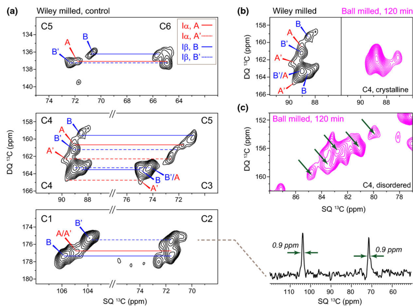
Fig. 3. High-resolution structural insights of cellulose in unlabeled cotton. (a) Resonance assignments of I\alpha and I\beta signals in Wiley-milled cotton. Representative ^{13}\text{C} cross section shows a typical ^{13}\text{C} linewidth is 0.9-1.0 ppm. The double-quantum and single-quantum chemical shifts are abbreviated as DQ and SQ, respectively. (b) The crystalline region of cellulose is altered after 2 h of ball-milling. The spectral features of I\alpha and I\beta cellulose in the control Wiley-milled sample are fully removed in the ball-milled sample. (c) The C4 region of disordered cellulose in ball-milled sample resolved five sub-forms as indicated using arrows
