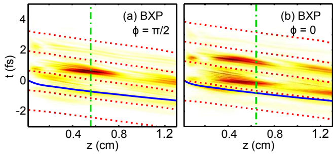
Figure 2: (Color Online) Axial time profile (linear scale) of the harmonic field versus propagation distance z for the BXP case for initial CEP (a) \phi = \pi/2 and (b) \phi = 0 , synthesized with no further spectral filtering other than a high-pass filter \omega > 10\omega_0 . The solid blue curves and the dashed red curves show the propagation of the center of mass (envelope peak) and the positions of squared field maxima of the driving infrared pulse, respectively. The vertical dashed-dotted lines mark the z positions of lowest ratio between the second most intense peak and the main peak for the \phi = \pi/2 case and the propagation distance chosen for Fig. 4(b) in the \phi = 0 case.
