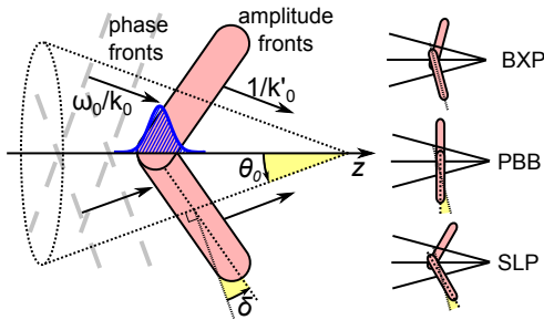
Figure 1: (Color Online) Schematic propagation of a CW: the gray dashed lines represent phase fronts and the red areas amplitude fronts. \theta_0 and \delta are the propagation and tilt angles, respectively. Note that the quantities v_p and v_e refer to the main intensity peak of the pulse, represented in the figure by the blue Gaussian profile. On the right there is a schematic representation of the PBB, BXP and SLP cases, as defined in the text.
