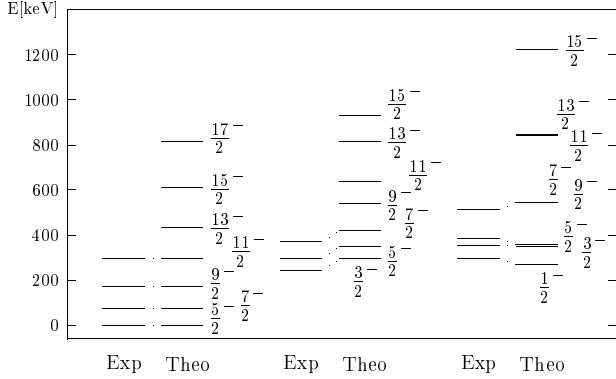
FIG. 2. Energy spectra of ^{165}\text{Er} . ‘Exp’ represents the experimental results and ‘Theo’ the calculated ones.
