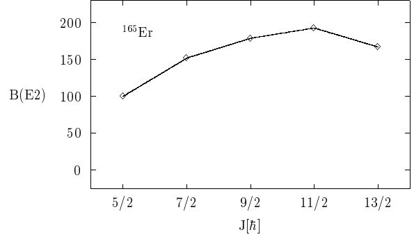
FIG. 4. Theoretical B(E2; J^- \rightarrow (J+2)^-) B(E2) trends in ^{165}\text{Er} [ e^2 b^2 \times 10^{-2} ].
