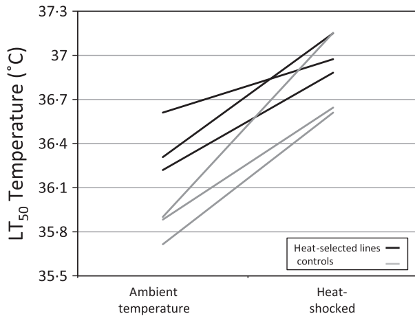
Fig. 3. Thermal tolerance ( LT_{50} ) in hybrid populations of Tigriopus californicus either selected for increased heat tolerance or held under the same conditions as unselected control lines. Figure shows heat tolerance for both sets of lines held at ambient temperature, and after being subjected to heat shock at 34 °C and allowed a 24-h recovery. A logistic regression analysis revealed an effect of selection ( P < 0.001 ) and prior heat shock ( P < 0.001 ) on thermal tolerance, but also a significant interaction between selection and heat shock ( P < 0.001 ) with a smaller effect of heat shock on thermal tolerance in selected lines.
