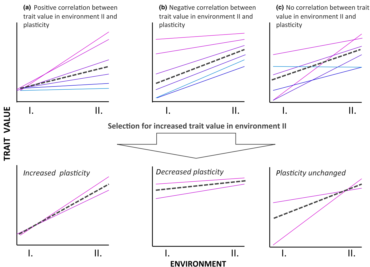
Fig. 1. Three scenarios for the relationship between phenotypic plasticity and trait means. Each line represents a reaction norm, trait values of an individual genotype in two or more environments. Reaction norms with steeper slopes indicate greater phenotypic plasticity. Dashed lines indicate the population mean. In scenario A, genotypes with the greatest trait mean in environment I also have the greatest plasticity, so that selection for increased trait values will lead to an increase in plasticity as a correlated response to selection. In scenario B, genotypes with the greatest trait values in environment II also have the lowest plasticity, leading to a decrease in plasticity as a correlated response to selection. Finally, scenario C posits no correlation between trait means and plasticities.
