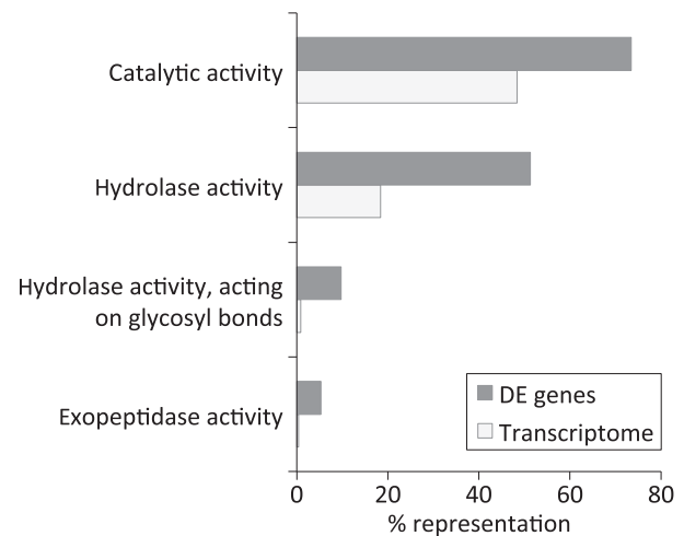
Fig. 5. Gene ontologies that were functionally enriched among transcripts responding to heat shock (Fisher's exact test, FDR = 0.05). Light bars show the percentage representation of ontologies in the transcriptome as a whole; dark bars show percentage representation within the differentially expressed transcripts.
