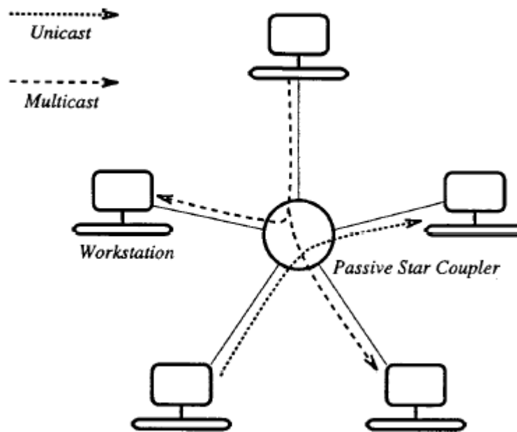
Figure 1.8 Broadcast and select networks.
