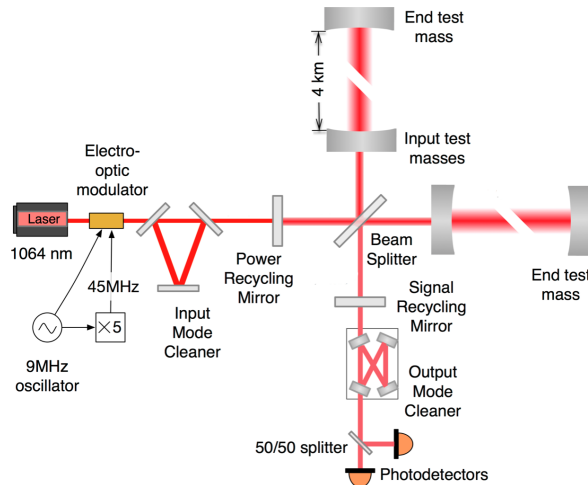
Figure 1: A schematic of aLIGO detectors taken from [6]
