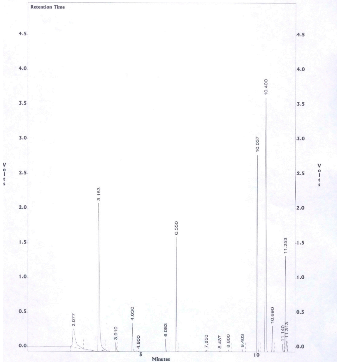
Figure 5.8: Gas Chromatograph of PFP derivatives of untreated day 15 shrimp extract on HP-225; putrescine, 10.03 min RT; cadaverine, 10.69 RT; hexanediamine, 11.14 RT.
