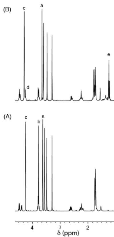
Figure 2. Proton NMR spectra, in CDCl 3 , of (A) chlorin e 6 trimethyl ester ( 6 ), and (B) chlorin e 6 15 2 -ethyl ester 13 1 ,17 3 -dimethyl ester ( 7 ). Assignments a 17 3 -OMe, b 15 2 -OMe, c 13 1 -OMe, d 15 2 -OCH 2 CH 3 , e 15 2 OCH 2 CH 3
