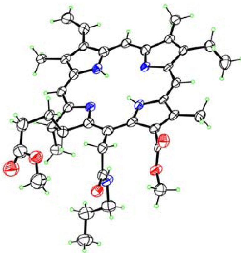
Figure 3. X-Ray structure of the 15 2 -monopropanamide-13 1 ,15 2 -dimethyl ester conjugate ( 8 ) of chlorin e 6 , one of four independent molecules, shown with 50% ellipsoids.
