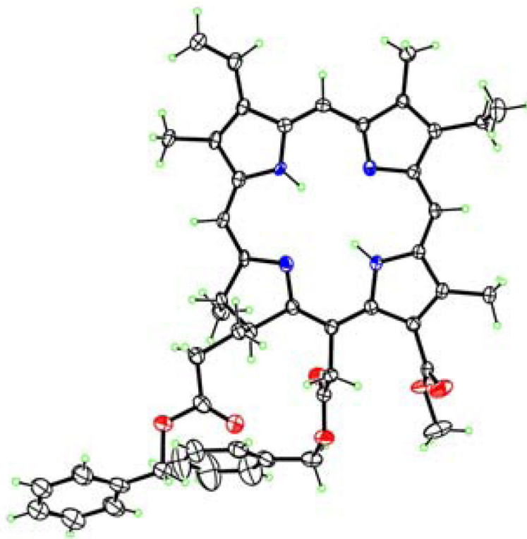
Figure 4. X-Ray structure of the chlorin e 6 15 2 ,17 3 -dibenzyl ester-13 1 -methyl ester ( 15 ); one of four independent molecules, shown with 50% ellipsoids.
