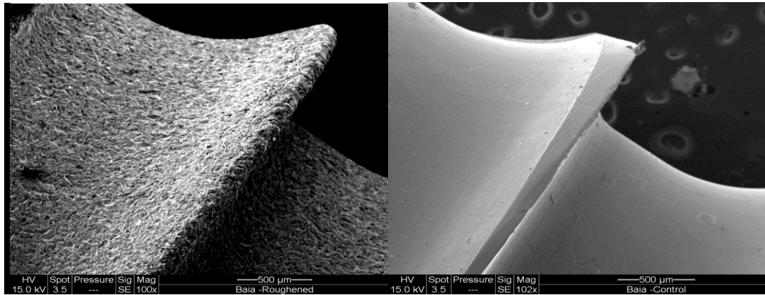
Figure 1.4 SEM picture of Al 2 O 3 roughened (R) and electroplished AO cortical screws (AO).
