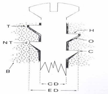
Figure 1.3 Diagram showing contact between screw and bone (B)-is limited at a part of the horizontal thread surface (H). The oblique (O) undersurface is separated by a space show as dark strip. When a tap (T) has been used to cut threads into cortical bone, the thread crest of the screw does not touch the bone. CD = core diameter; ED = thread diameter (Figure taken from Uthoff, 1973).
