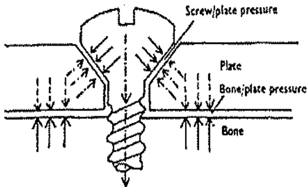
Figure 1.2 Schematic representation of compressive stresses between screw and plate countersink and between bone and plate, by the tensile stress induced in the screw. (Figure taken from Hughes et al. 1972)
