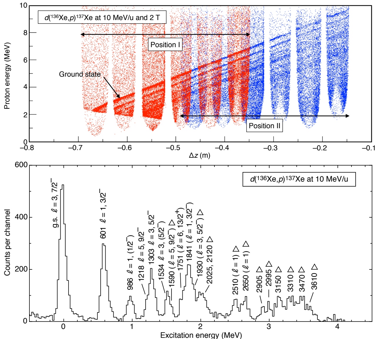
FIG. 2. (Color online) (Top) Proton energy versus longitudinal distance traveled between the target and the point of impact on the Si array, \Delta z , for the d(^{136}\text{Xe},p)^{137}\text{Xe} reaction at 10 MeV/u and a 2-T field. The plot is a composite of two different target positions, as discussed in the text. (Bottom) Representative proton spectrum. Peaks are labeled by their energy (to the nearest keV) and by their \ell value, spin and parity, where these quantities are known. States marked with a \Delta symbol are those with energy, \ell value, or both, deduced for the first time in this work. A smooth background has been subtracted to produce the displayed spectrum as discussed in the text.
