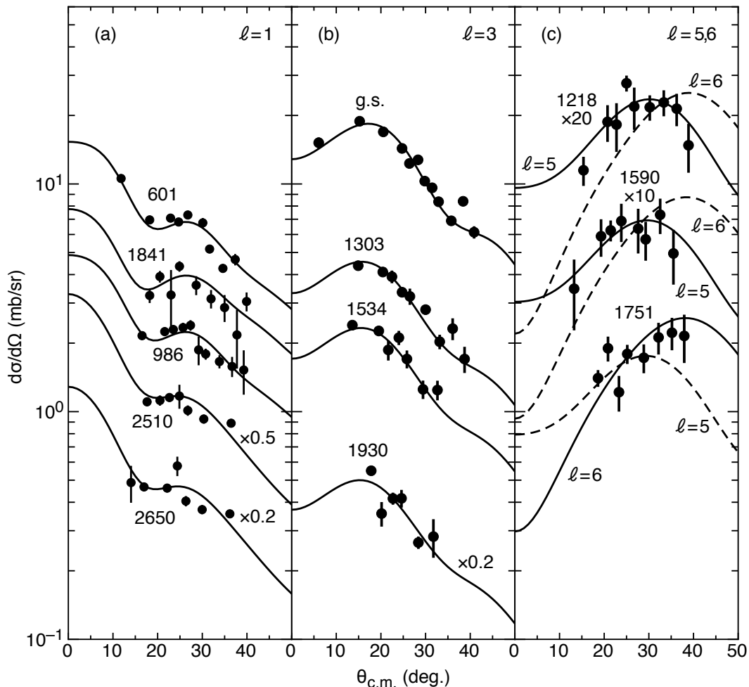
FIG. 3. (Color online) Angular distributions for the outgoing protons in the d(^{136}\text{Xe},p)^{137}\text{Xe} reaction. Panels (a), (b) and (c) group the \ell = 1, 3, 5 and 6 angular distributions, respectively. Some data have been scaled by a multiplicative factor, labeled on the plots. The solid circles represent the data – the error bars convey the statistical uncertainty – whilst the curves are DWBA calculations normalized to fit the data. States are labeled by their energy in keV and their assigned \ell value. For the high- \ell transfer, where the angular distributions for \ell = 5 and 6 are similar, both fits are shown; the best fit as a solid line, the other as a dashed line.
