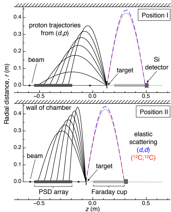
FIG. 1. (Color online) Schematic of the detector and target arrangements in HELIOS. Positions I and II are discussed in the text. The beam enters, on axis, from the left. The radial distance, r , and longitudinal coordinate, z , are given for sample proton trajectories (solid lines). Trajectories of elastically scattered ions, used for monitoring luminosity, are shown by dashed lines for deuterons (blue online), and dotted lines for ^{12}\text{C} ions (red online). The z axis is both the beam axis and the magnetic axis where z = 0.0 m is the center of the solenoid.
