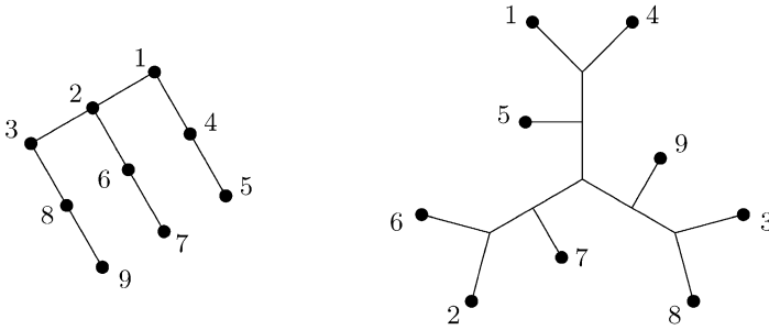
FIG. 3. (a) The matroid M_9 . (b) A width-3 branch decomposition of M_9 .
