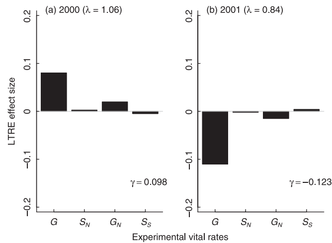
Fig. 4 Life Table Response Experiment (LTRE) analysis by year for a) 2000 and b) 2001 with their corresponding dominant eigenvalue ( \lambda ) and total contribution for individual years ( \gamma ). Terms on the x-axis represent germination rate ( G ), seedling survival ( S_N ), seedling growth to a flowering adult ( G_N ) and oversummer survival ( S_S ). All other vital rates were derived from field and glasshouse measurements and did not vary across treatments.
