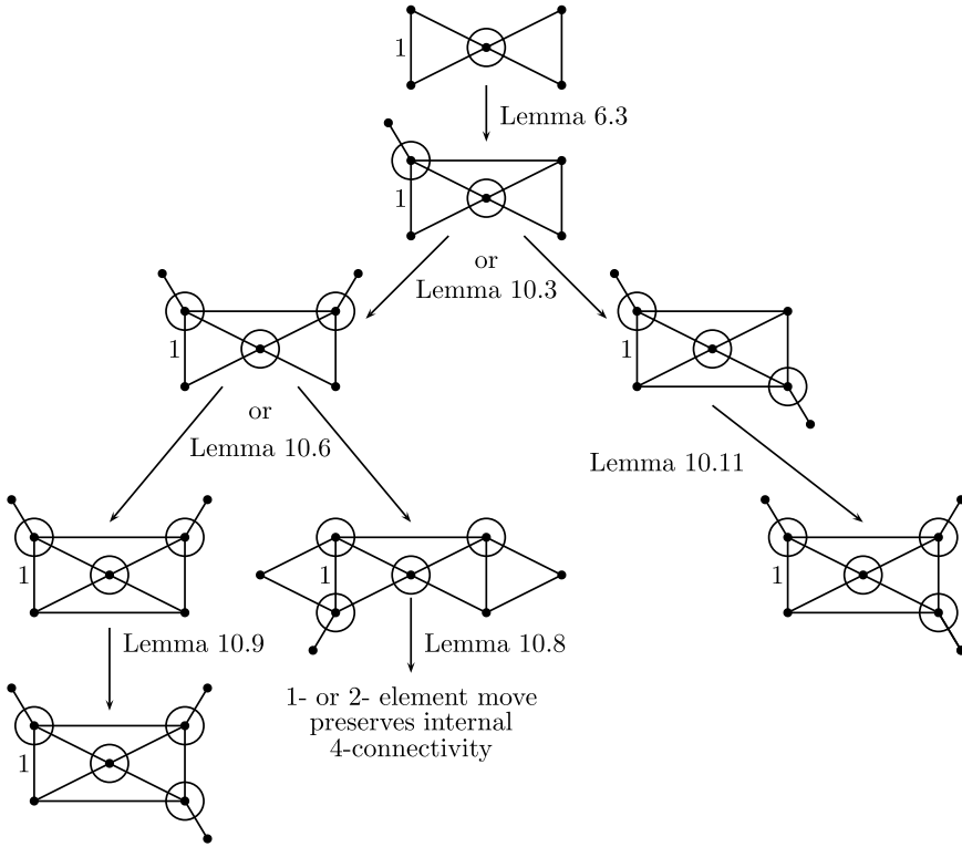
Fig. 5. The steps when M \setminus 1 has a unique 4-element fan.
