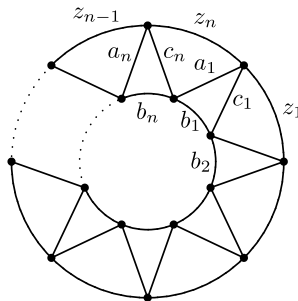
Fig. 13. A labelled quartic ladder.
