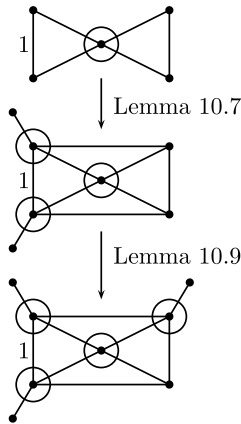
Fig. 6. When M \setminus 1 has more than one 4-element fan.
