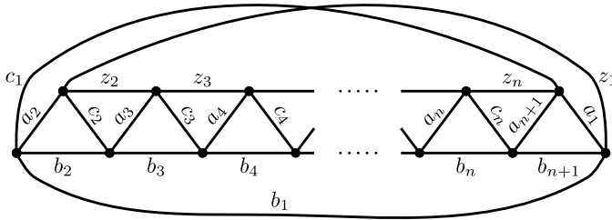
Fig. 18. A labelled quartic Möbius ladder.
