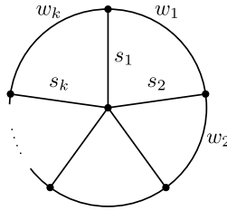
Fig. 8. A labelled wheel.
