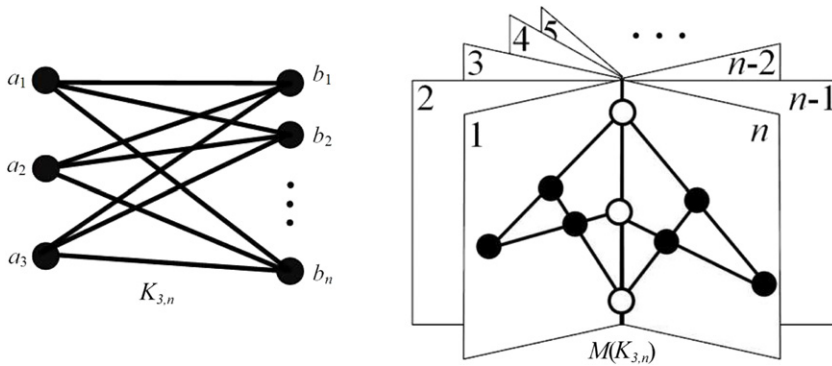
Fig. 6. The graph K_{3,n} and the geometry of M(K_{3,n}) with white dots representing points that are not present in the matroid.
