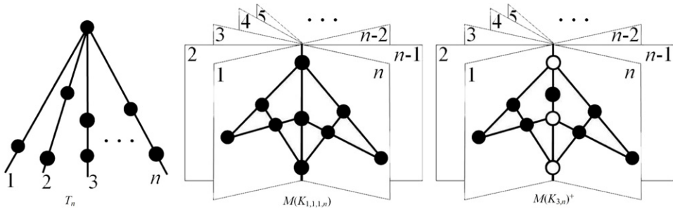
Fig. 2. Geometric illustrations of three matroids: T_n is the rank- n free spike with a tip and a cotip; M(K_{1,1,1,n}) and M(K_{3,n})^+ have rank n + 2 with the white dots representing points that are not present in the matroid.
