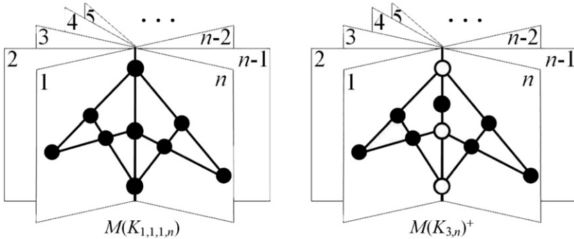
Fig. 7. Geometric representations of M(K_{1,1,1,n}) and M(K_{3,n})^+ .
