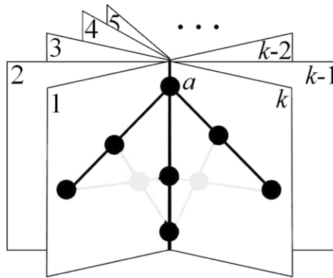
Fig. 8. Geometric representation of M(K_{1,1,k+1}) in rank k + 1 .
