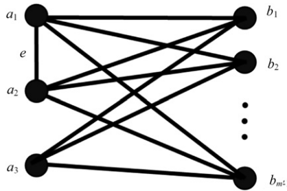
Fig. 9. The graph K'_{3,m^5-1} .
