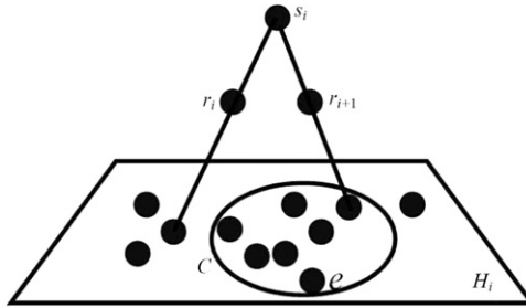
Fig. 5. The triad T_i^* = \{r_i, s_i, r_{i+1}\} and the complementary hyperplane H_i .
