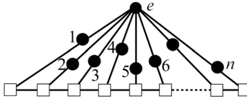
Fig. 3. Geometric illustration of N in rank 3. Possible lines containing subsets of [n] have not been shown.
