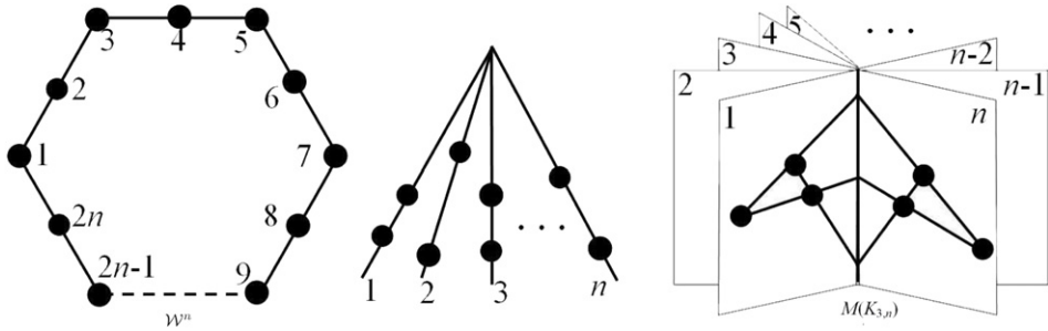
Fig. 1. Geometric illustrations of three of the unavoidable minors: the rank- n whirl, \mathcal{W}^n ; the rank- n tipless free spike; and M(K_{3,n}) , which has rank n + 2 .
