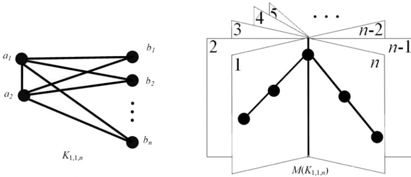
Fig. 4. The graph of K_{1,1,n} and the geometry of M(K_{1,1,n}) in rank n + 1 .
