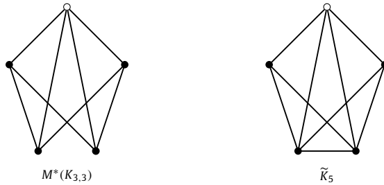
Fig. 3. Graft representations of M^*(K_{3,3}) and \tilde{K}_5 .
