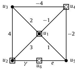
Fig. 14. Hypergraph representation (H', \{5, -3\}) of M_e^* , where 5 is incident with colored vertices and -3 is incident with boxed vertices.
