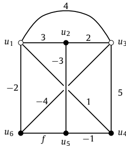
Fig. 15. Graft representation (H', \gamma) of M_f^* .
