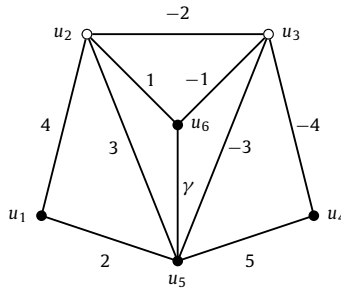
Fig. 10. A graft representation, (H', a) , of M_a^* , where a is incident with colored vertices.
