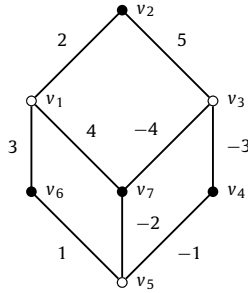
Fig. 9. A graft (G, \gamma) such that M(G, \gamma) \cong \tilde{K}_5^* .
