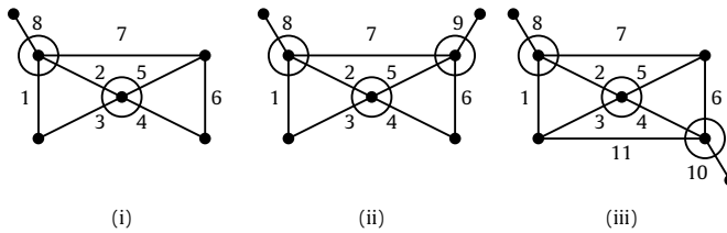
Fig. 6. Structure diagrams for (5). Note (iii) is also the diagram for (7).
