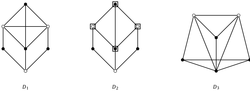
Fig. 2. Graft representations of D_1 , D_2 , and D_3 .
