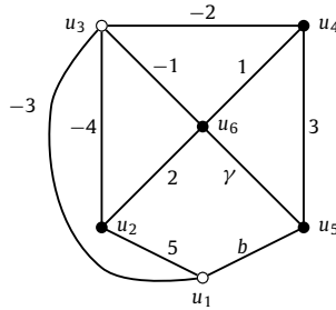
Fig. 11. Graft representation (H', 4) of M_b^* , where 4 is incident with colored vertices.
