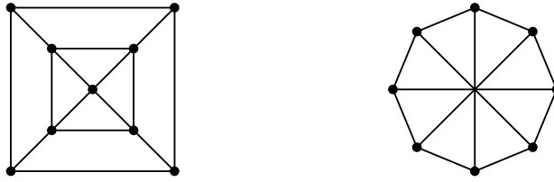
Fig. 1. The terrahawk, and the Wagner graph.
