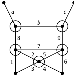
Fig. 7. Structure diagram for (6).
