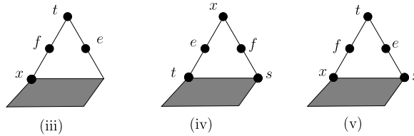
Fig. 1. Cases (iii), (iv), and (v) of Theorem 2.1.
