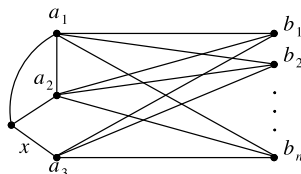
Fig. 11. A graph G representing M^* .
