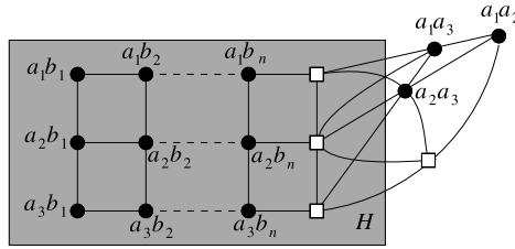
Fig. 10. M \setminus x with boxes representing the four possible locations for x .
