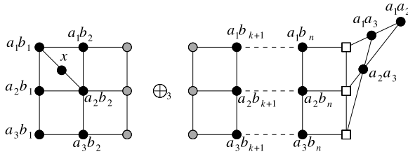
Fig. 12. M_0 shown as a 3-sum across the gray triangle when i = 2 .
