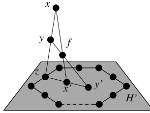
Fig. 6. Geometric illustration of M^* with x', y' , and z added to produce the matroid M_4 . Here H' is the complement of triad \{x, f, y\} .
