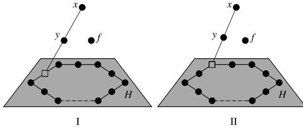
Fig. 2. Geometric illustration of M^* for cases I and II.
