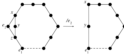
Fig. 4. Geometric illustration of one possible configuration of M_3 .
