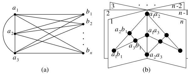
Fig. 8. (a) K_{1,1,1,n} and (b) a geometric illustration of M(K_{1,1,1,n}) .
