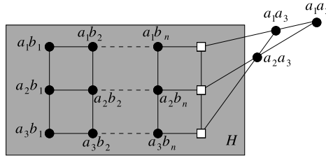
Fig. 9. A geometric illustration of M^*(K_{1,1,1,n}) .
