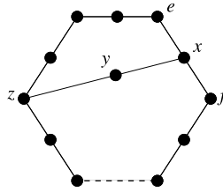
Fig. 3. Geometric illustration of M_2 .
