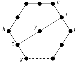
Fig. 5. Geometric illustration of M_3 .
