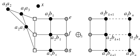
Fig. 13. The matroid M_1 with cocircuit \{x, a_1a_2, a_1a_3, a_2a_3\} illustrated as a 3-sum.
