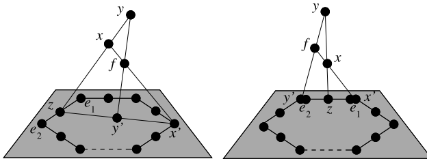
Fig. 7. Geometric illustration of M_5 (left) and one of its minors (right).
