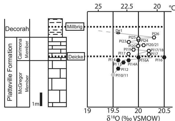
Figure 1. Plot of samples PI10/11 through De1 from Buggisch et al. (2010). PI samples are from the Cummingsville Annex Section; stratigraphy is from Webers (1966). Note that, using the correct placement of samples with regard to Deicke K-bentonite (DKb) bed, the cooling event occurred prior to the volcanic eruption. Black solid polygons are samples from below the DKb, black open polygons are samples above the DKb within the Carimona; oval is the first sample within the Decorah. Lowermost sample (gray polygon) reported in the supplementary data set of Buggisch et al. (2010, GSA Data Repository item 2010087) is PI10/11, but it apparently was not plotted in their figures. Additionally, this sample (PI10/11) is listed as 3.50 m in the supplementary data set, but according to the Webers (1966) stratigraphy, is at ~6.46 m.
