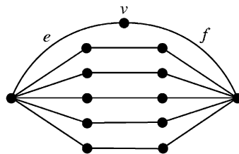
Fig. 1. D is the union of C_{3,3}^* , e , and f .
