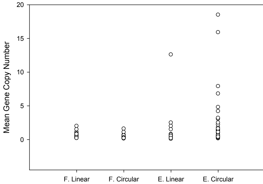
Figure 3.5 Mean gene copy number from technical replicates of isolated single cell colonies.
