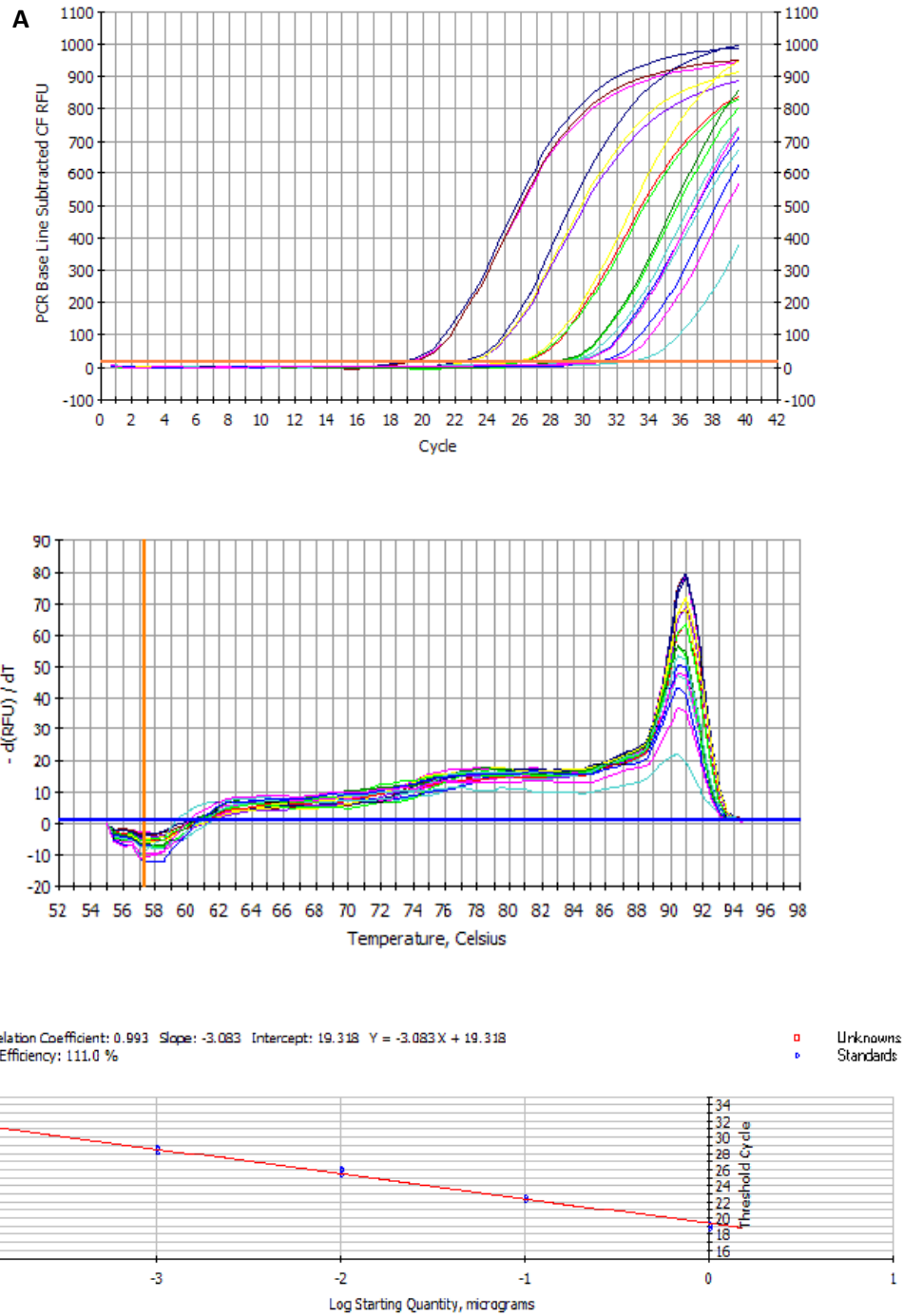
Figure 3.2 Dilution Ct values, melting curves, and standard curve obtained from the optimization of the forward and reverse primers. Five 10 fold dilutions (exogenous DNA equivalent to 1 \times 10^3 to 1 \times 10^7 cells) were used to generate the dilution curves: (A), melt curve data (B), and standard curve (C).
