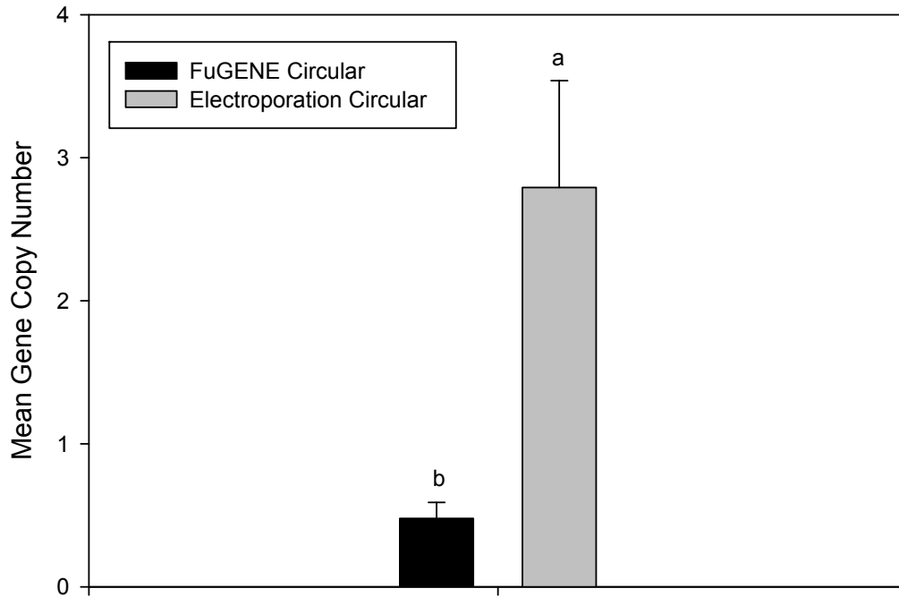
A3 Mean gene copy number for FuGENE ® HD and electroporation circular. Bars indicated \pm SEM. Statistical difference were determined by One-Way ANOVA ( P < 0.05 ).
