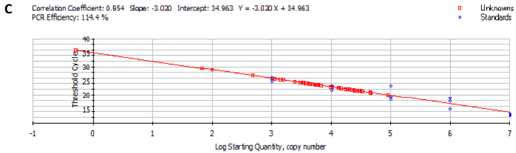
Figure 3.3 Ct values (A), melting curves (B), and standard curve (C) obtained when sample are amplified. All samples, including the no template negative control were run in triplicates and compared to a standard curve developed by a 10 fold serial dilution.
