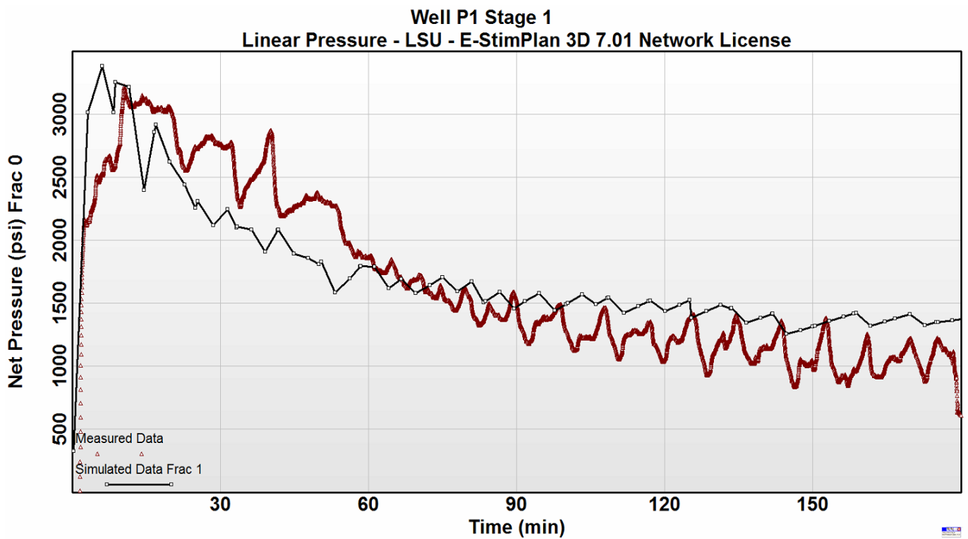
Figure 5.4a. Forward modeling of stage1of fracturing treatments with orthogonal natural fractures
