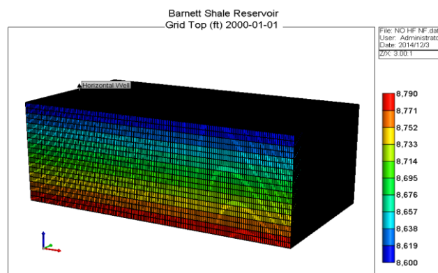
Figure 6.1. GEM-type reservoir model in CMG
