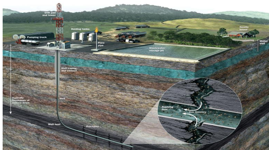
Figure 1.1. Schematic of Hydraulic Fracturing
