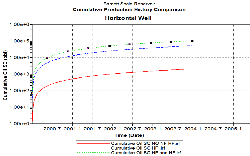
Figure 6.10. Production enhancements from hydraulic fracturing and natural fractures for shale oil reservoir
