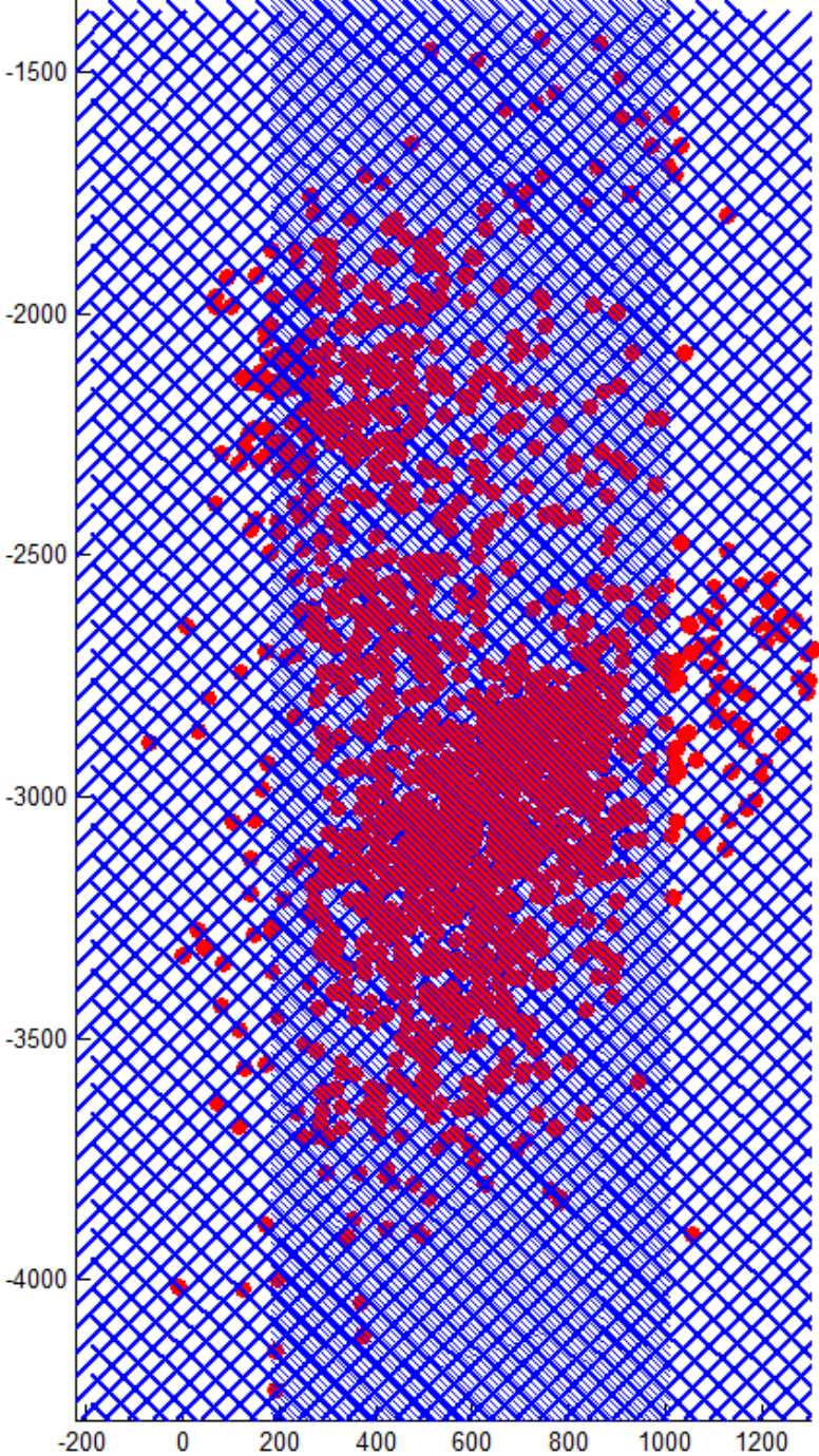
Figure 4.15. Adaptive spacing algorithm for non-orthogonal natural fractures, which also generated finer gridding systems and smaller overall squared error.
