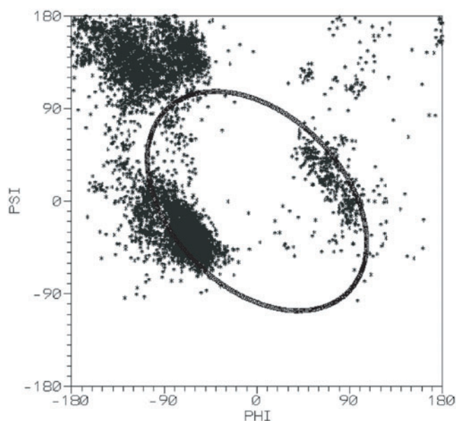
Fig. 1. The ellipse-path limited conformational sub-space in relation to Phi, Psi angles as they appear in real proteins. The shortest distance between particular Phi, Psi angles and ellipse-belonging point represents the way in which the Phi, Psi angles on the ellipse can be found.
