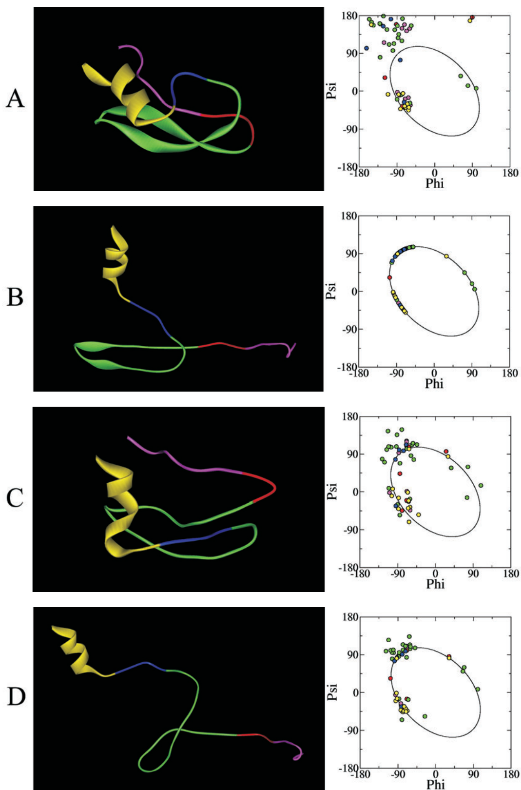
Fig. 2. The structure of BPTI and its Phi, Psi angles distribution versus ellipse-path (A) native form, (B) ellipse-based structure, (C) post-energy-minimization structure of BPTI with SS-bonds present in procedure, (D) post-energy-minimization structural form of BPTI with SS-bonds absent in procedure.
