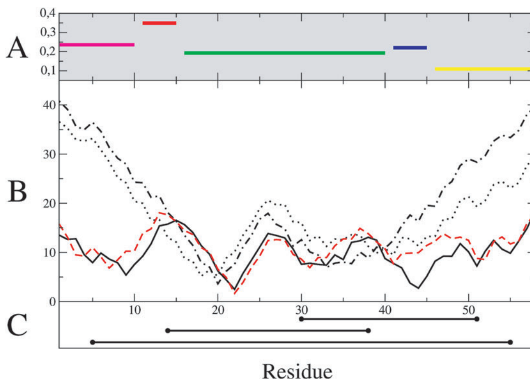
Fig. 3. The comparison of structural forms of BPTI protein molecule. (A) RMS-D (per residue) calculated for structurally differentiated polypeptide fragments. The fragments were defined according to the profile presented in B . The parallel fragments of curves represent the correct spatial orientation of the polypeptide, while the dissimilar regularity of the curve represents fragments with low similarity of the spatial orientation of the particular polypeptide fragment. (B) Profile representing the distribution of distances linking the geometrical center of the molecule with sequential C\alpha atoms. Continuous line—native form, Dotted line—ellipse-derived structure, Dashed red line—post-energy-minimization structure with SS-bonds present, Dotted/dashed line—post-energy-minimization structure with SS-bonds absent. (C) SS-bonds system in BPTI. The color notation introduced in all graphical presentations in this paper in accordance to fragments distinguished in this figure.
