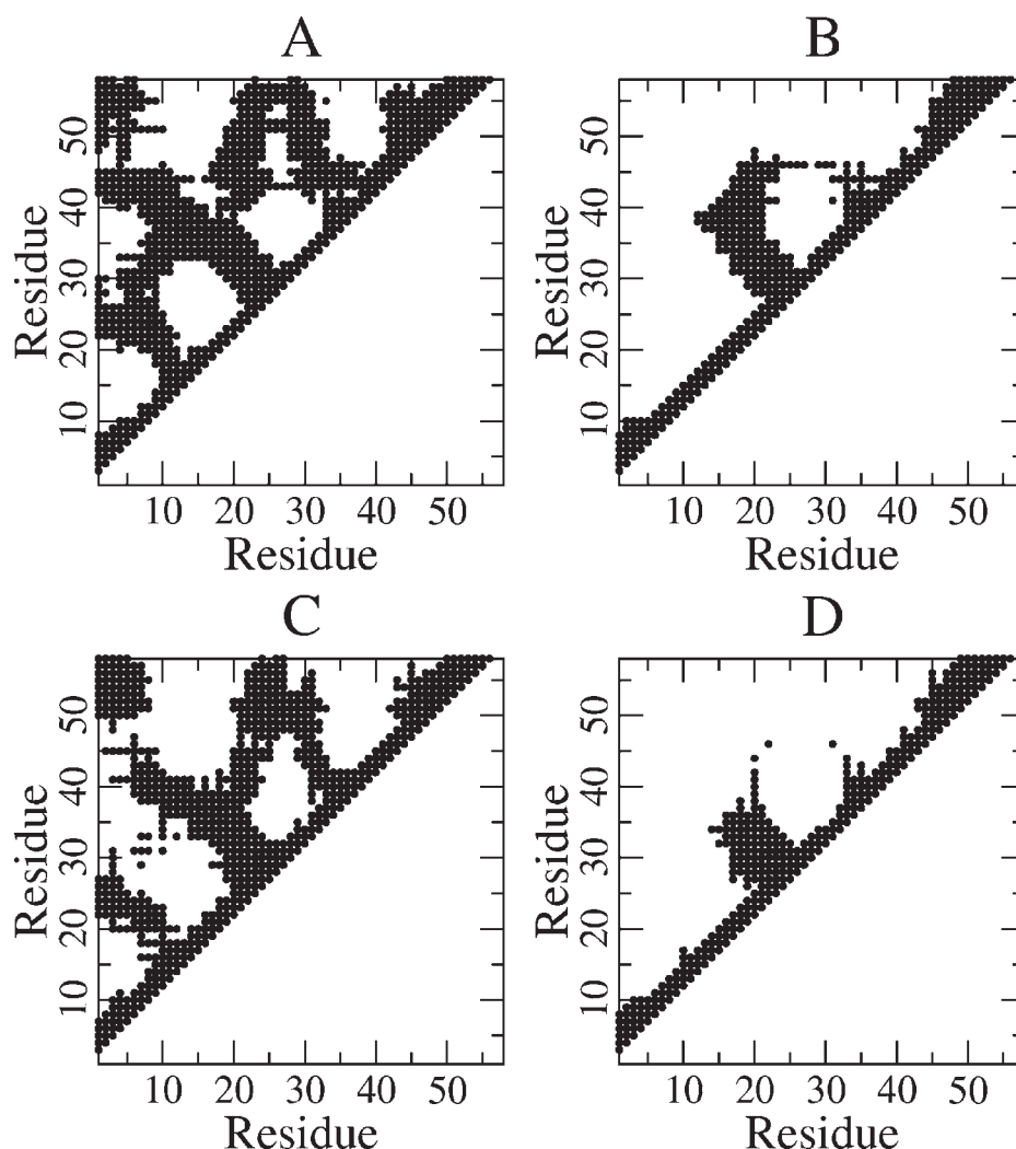
Fig. 4. Non-bonding contacts in BPTI: (A) Native form, (B) ellipse-derived structure, (C) post-energy-minimization with SS-bonds present, (D) post-energy-minimization with SS-bonds absent.
