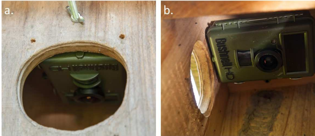
Figure 1. Modified Bushnell Nature View trail camera equipped with an Alilusso 7.5mm iPhone fisheye lens used to monitor nest boxes for wood ducks ( Aix sponsa ). Cameras were mounted inside nest boxes using a threaded rod and wing nut (a) providing a top-down view inside (b).
